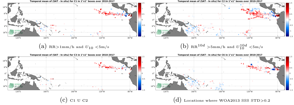
Figure 11: Temporal mean gridded over spatial boxes of size 1^\circ \times 1^\circ of \Delta SSS (SMOS-L3-CATDS-CECOS-LOCEAN-V3-18DAYS-25KM - Surface drifters) for 4 different subdatasets corresponding to: RR > 1\text{mm/h} and U_{10} < 5\text{m/s} (a), RR^{10d} > 5\text{mm/h} and U_{10}^{10d} < 5\text{m/s} (b), C1 U C2 (c), Locations where WOA2013 SSS STD > 0.2 (d).
