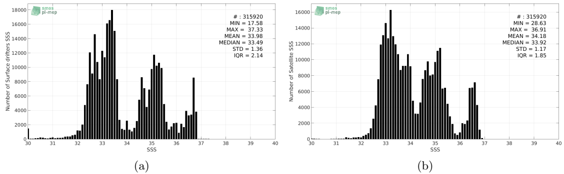
Figure 2: Histograms of SSS from Surface drifters (a) and SMOS-L3-CATDS-CECOS-LOCEAN-V3-18DAYS-25KM (b) considering all match-up pairs per bins of 0.1 over the Tropical Pacific Ocean Pi-MEP region and for the full satellite product period.
