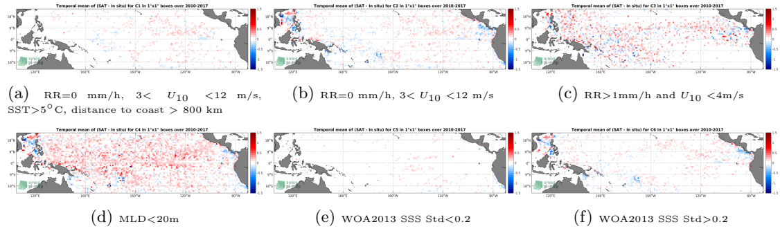
Figure 12: Temporal mean gridded over spatial boxes of size 1^\circ \times 1^\circ of \Delta SSS (SMOS-L3-CATDS-CECOS-LOCEAN-V3-18DAYS-25KM - Argo) for 6 different subdatasets corresponding to: RR=0 mm/h, 3 < U_{10} < 12 m/s, SST > 5^\circ C , distance to coast > 800 km (a), RR=0 mm/h, 3 < U_{10} < 12 m/s (b), RR > 1 mm/h and U_{10} < 4 m/s (c), MLD < 20 m (d), WOA2013 SSS Std < 0.2 (e), WOA2013 SSS Std > 0.2 (f).
