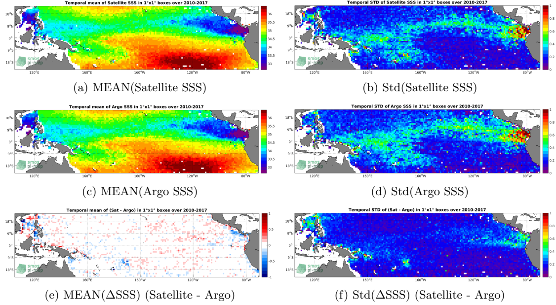
Figure 6: Temporal mean (left) and Std (right) of SSS from SMOS-L3-CATDS-CECOS-LOCEAN-V3-18DAYS-25KM (top), Argo (middle), and of \Delta SSS (Satellite - Argo). Only match-up pairs are used to generate these maps.
