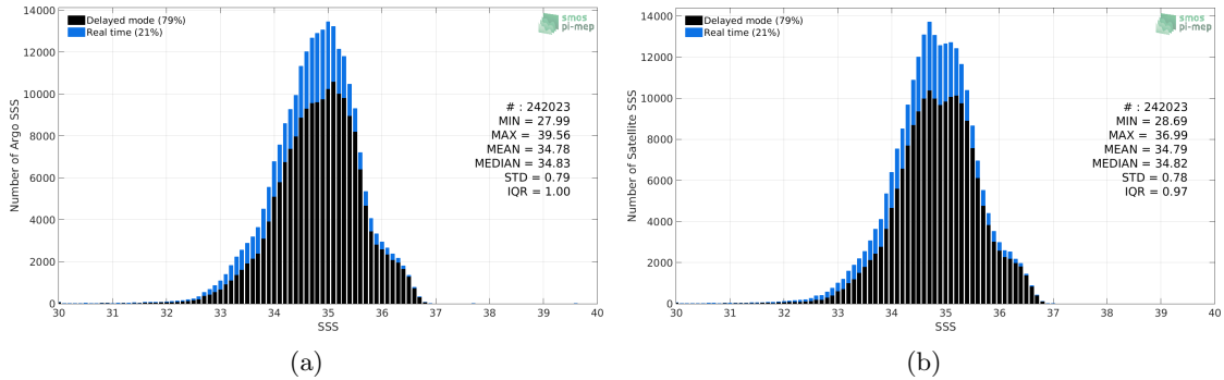
Figure 2: Histograms of SSS from Argo (a) and SMOS-L3-CATDS-CECOS-LOCEAN-V3-18DAYS-25KM (b) considering all match-up pairs per bins of 0.1 over the Tropical Pacific Ocean Pi-MEP region and for the full satellite product period.
