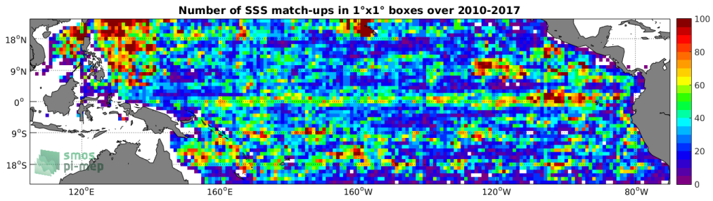
Figure 4: Number of SSS match-ups between Argo SSS and the SMOS-L3-CATDS-CECOS-LOCEAN-V3-18DAYS-25KM SSS product for the Tropical Pacific Ocean Pi-MEP region over 1^\circ \times 1^\circ boxes and for the full satellite product period.
