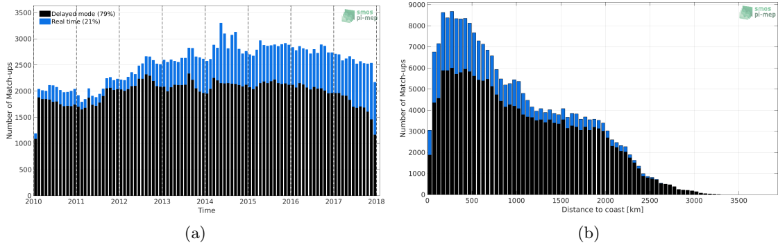
Figure 1: Number of match-ups between Argo and SMOS-L3-CATDS-CECOS-LOCEAN-V3-18DAYS-25KM SSS as a function of time (a) and as function of the distance to coast (b) over the Tropical Pacific Ocean Pi-MEP region and for the full satellite product period.
