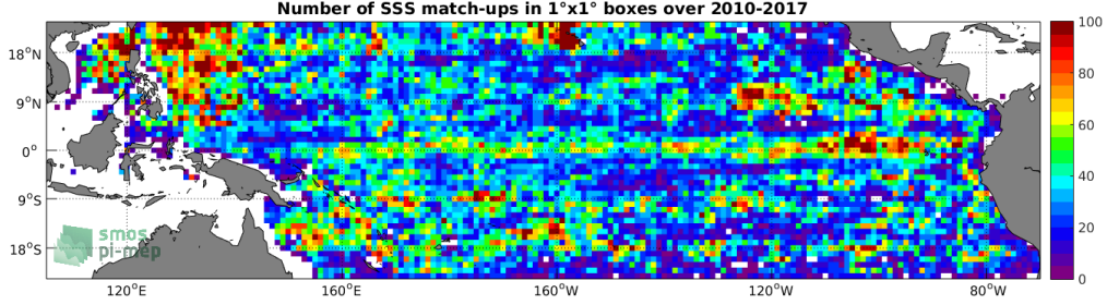
Figure 4: Number of SSS match-ups between Argo SSS and the SMOS-L3-CATDS-CECOS-LOCEAN-V3-18DAYS-25KM SSS product for the Tropical Pacific Ocean Pi-MEP region over 1^\circ \times 1^\circ boxes and for the full satellite product period.
