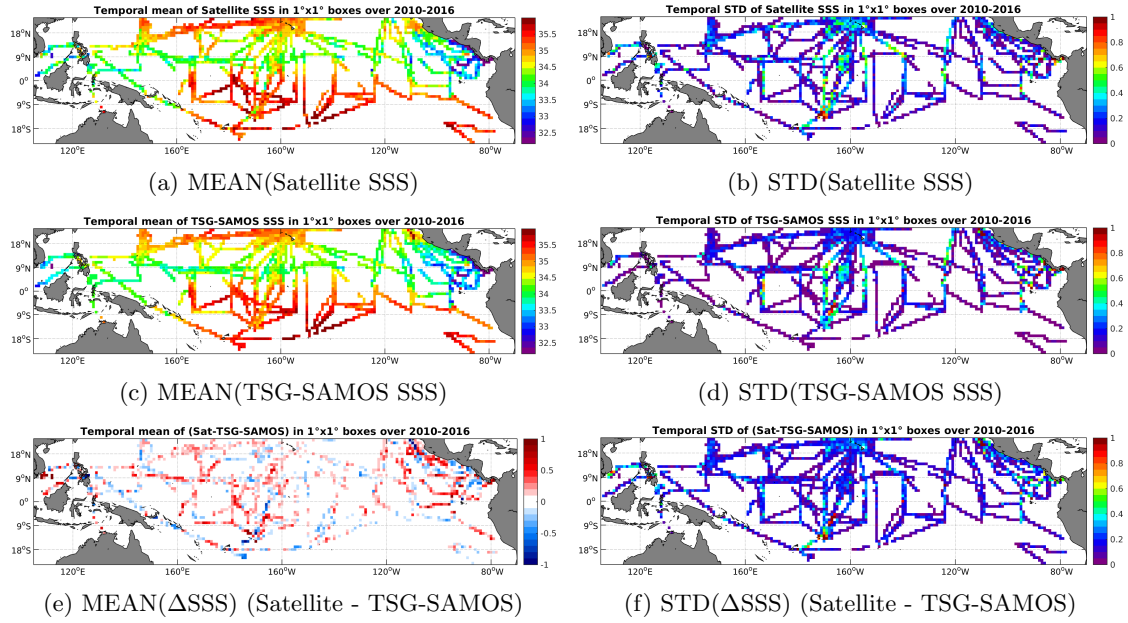
Figure 6: Temporal mean (left) and STD (right) of SSS from SMOS-L3-CATDS-CECOS-LOCEAN-V2-9DAYS-25KM (top), TSG-SAMOS (middle), and of \Delta SSS (Satellite - TSG-SAMOS). Only match-up pairs are used to generate these maps.
