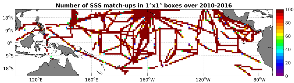
Figure 4: Number of SSS match-ups between TSG-SAMOS SSS and the SMOS-L3-CATDS-CECOS-LOCEAN-V2-9DAYS-25KM SSS product for the Tropical Pacific Ocean Pi-MEP region over 1^\circ \times 1^\circ boxes and for the full satellite product period.
