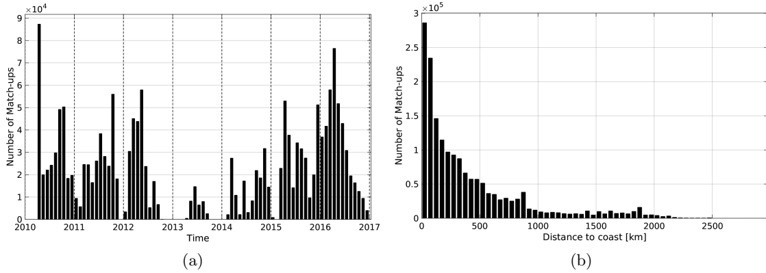
Figure 1: Number of match-ups between TSG-SAMOS and SMOS-L3-CATDS-CECOS-LOCEAN-V2-9DAYS-25KM SSS as a function of time (a) and as function of the distance to coast (b) over the Tropical Pacific Ocean Pi-MEP region and for the full satellite product period.
