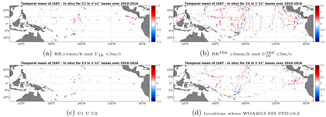
Figure 12: Temporal mean gridded over spatial boxes of size 1^\circ \times 1^\circ of \Delta SSS (SMOS-L3-CATDS-CECOS-LOCEAN-V2-9DAYS-25KM - TSG-SAMOS) for 4 different subdatasets corresponding to: RR > 1\text{mm/h} and U_{10} < 5\text{m/s} (a), RR^{10d} > 5\text{mm/h} and U_{10}^{10d} < 5\text{m/s} (b), C1 U C2 (c), Locations where WOA2013 SSS STD > 0.2 (d).
