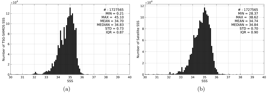
Figure 2: Histograms of SSS from TSG-SAMOS (a) and SMOS-L3-CATDS-CECOS-LOCEAN-V2-9DAYS-25KM (b) considering all match-up pairs per bins of 0.1 over the Tropical Pacific Ocean Pi-MEP region and for the full satellite product period.
