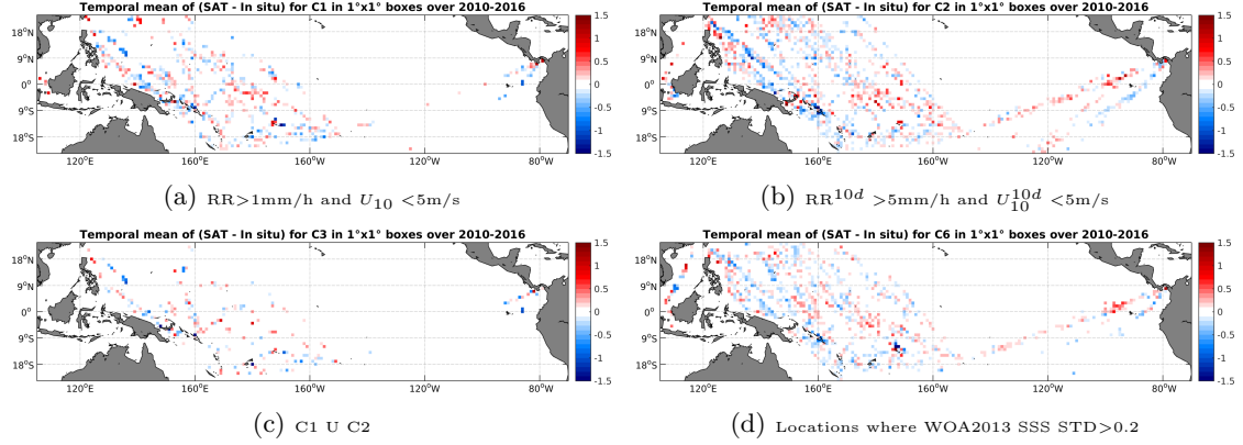
Figure 12: Temporal mean gridded over spatial boxes of size 1^\circ \times 1^\circ of \Delta SSS (SMOS-L3-CATDS-CECOS-LOCEAN-V2-9DAYS-25KM - TSG-LEGOS-DM) for 4 different subdatasets corresponding to: RR > 1\text{mm/h} and U_{10} < 5\text{m/s} (a), RR^{10d} > 5\text{mm/h} and U_{10}^{10d} < 5\text{m/s} (b), C1 U C2 (c), Locations where WOA2013 SSS STD > 0.2 (d).
