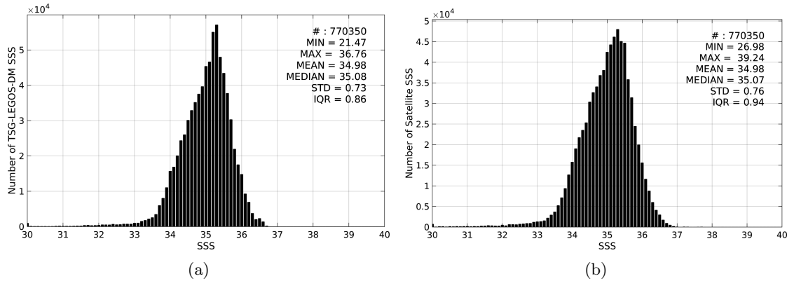
Figure 2: Histograms of SSS from TSG-LEGOS-DM (a) and SMOS-L3-CATDS-CECOS-LOCEAN-V2-9DAYS-25KM (b) considering all match-up pairs per bins of 0.1 over the Tropical Pacific Ocean Pi-MEP region and for the full satellite product period.
