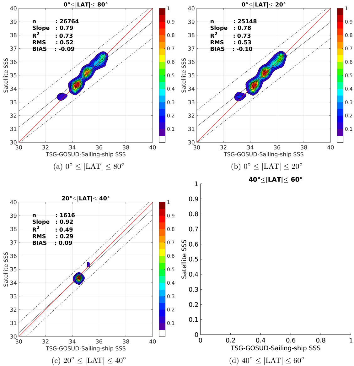
Figure 9: Contour maps of the concentration of SMOS-L3-CATDS-CECOS-LOCEAN-V2-9DAYS-25KM SSS (y-axis) versus TSG-GOSUD-Sailing-ship SSS (x-axis) at match-up pairs for different latitude bands. For each plot, the red line shows x=y . The black thin and dashed lines indicate a linear fit through the data cloud and the \pm 95\% confidence levels, respectively. The number match-up pairs n , the slope and R^2 coefficient of the linear fit, the root mean square (RMS) and the mean bias between satellite and in situ data are indicated for each latitude band in each plots.
