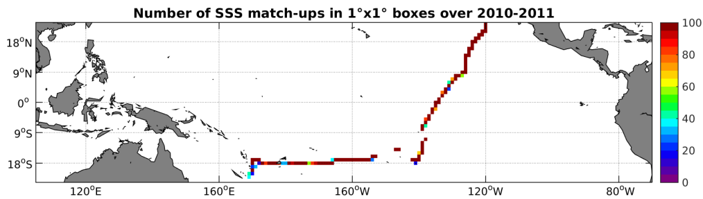
Figure 4: Number of SSS match-ups between TSG-GOSUD-Sailing-ship SSS and the SMOS-L3-CATDS-CECOS-LOCEAN-V2-9DAYS-25KM SSS product for the Tropical Pacific Ocean Pi-MEP region over 1^\circ \times 1^\circ boxes and for the full satellite product period.
