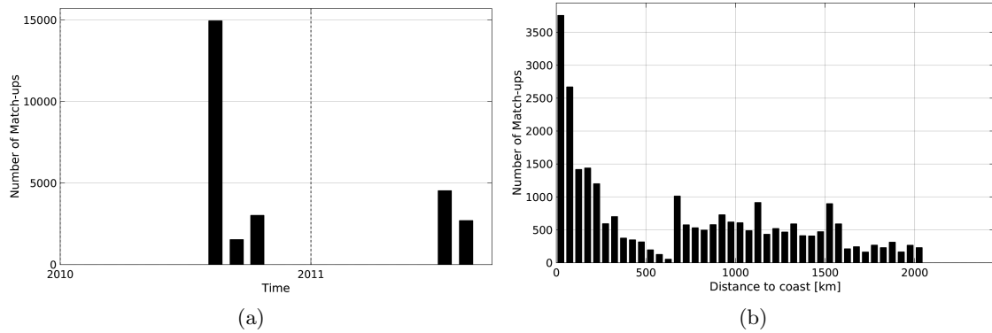
Figure 1: Number of match-ups between TSG-GOSUD-Sailing-ship and SMOS-L3-CATDS-CECOS-LOCEAN-V2-9DAYS-25KM SSS as a function of time (a) and as function of the distance to coast (b) over the Tropical Pacific Ocean Pi-MEP region and for the full satellite product period.
