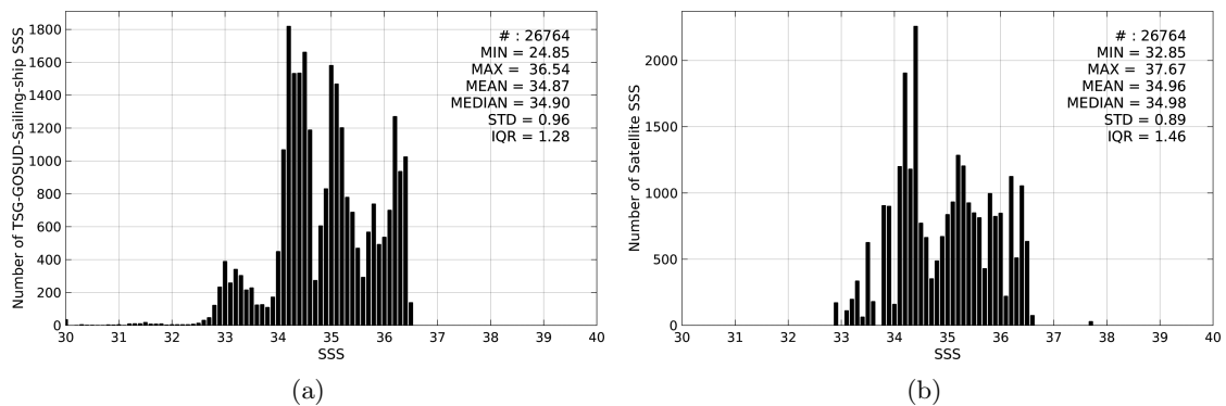
Figure 2: Histograms of SSS from TSG-GOSUD-Sailing-ship (a) and SMOS-L3-CATDS-CECOS-LOCEAN-V2-9DAYS-25KM (b) considering all match-up pairs per bins of 0.1 over the Tropical Pacific Ocean Pi-MEP region and for the full satellite product period.
