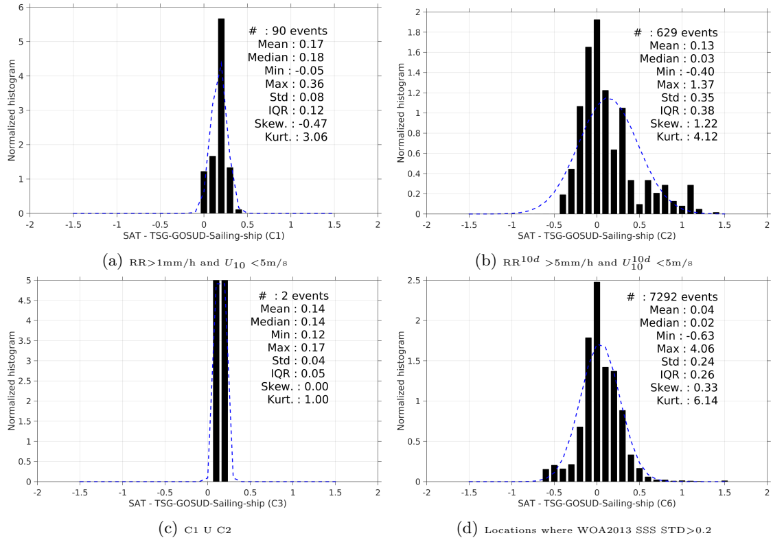
Figure 13: Normalized histogram of \Delta SSS (SMOS-L3-CATDS-CECOS-LOCEAN-V2-9DAYS-25KM - TSG-GOSUD-Sailing-ship) for 6 different subdatasets corresponding to: RR > 1mm/h and U_{10} < 5 m/s (a), RR^{10d} > 5 mm/h and U_{10}^{10d} < 5 m/s (b), C1 U C2 (c), Locations where WOA2013 SSS STD > 0.2 (d).
