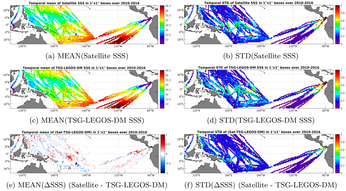
Figure 6: Temporal mean (left) and STD (right) of SSS from SMOS-L3-CATDS-CECOS-LOCEAN-V2-18DAYS-25KM (top), TSG-LEGOS-DM (middle), and of \Delta SSS (Satellite - TSG-LEGOS-DM). Only match-up pairs are used to generate these maps.
