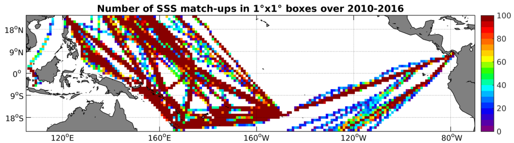
Figure 4: Number of SSS match-ups between TSG-LEGOS-DM SSS and the SMOS-L3-CATDS-CECOS-LOCEAN-V2-18DAYS-25KM SSS product for the Tropical Pacific Ocean Pi-MEP region over 1^\circ \times 1^\circ boxes and for the full satellite product period.
