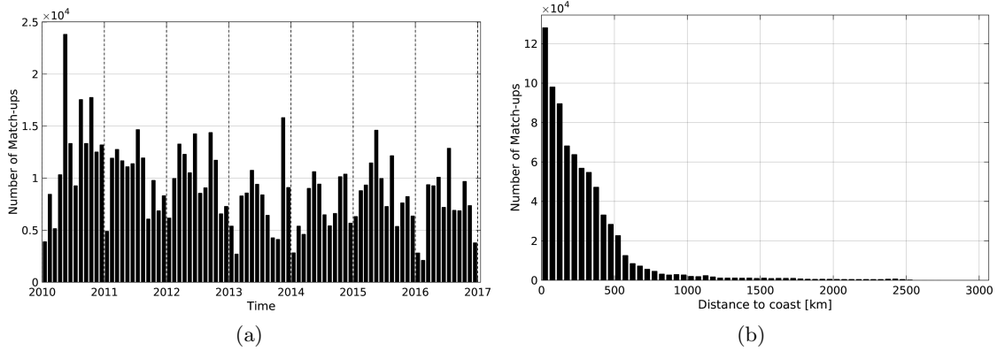
Figure 1: Number of match-ups between TSG-LEGOS-DM and SMOS-L3-CATDS-CECOS-LOCEAN-V2-18DAYS-25KM SSS as a function of time (a) and as function of the distance to coast (b) over the Tropical Pacific Ocean Pi-MEP region and for the full satellite product period.
