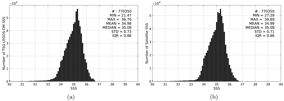
Figure 2: Histograms of SSS from TSG-LEGOS-DM (a) and SMOS-L3-CATDS-CECOS-LOCEAN-V2-18DAYS-25KM (b) considering all match-up pairs per bins of 0.1 over the Tropical Pacific Ocean Pi-MEP region and for the full satellite product period.
