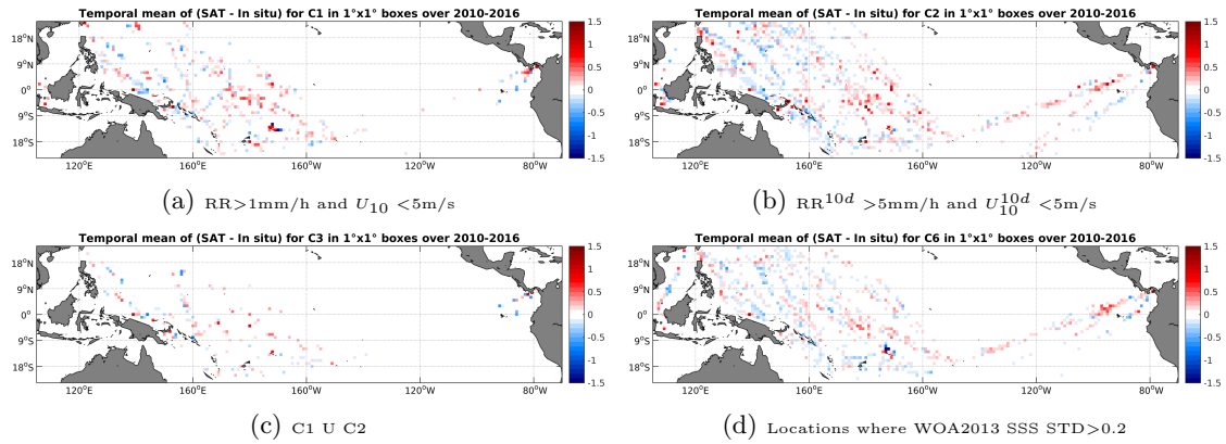
Figure 12: Temporal mean gridded over spatial boxes of size 1^\circ \times 1^\circ of \Delta SSS (SMOS-L3-CATDS-CECOS-LOCEAN-V2-18DAYS-25KM - TSG-LEGOS-DM) for 4 different subdatasets corresponding to:RR >1 mm/h and U_{10} < 5 m/s (a), RR 10d > 5 mm/h and U_{10}^{10d} < 5 m/s (b), C1 U C2 (c),Locations where WOA2013 SSS STD >0.2 (d).
