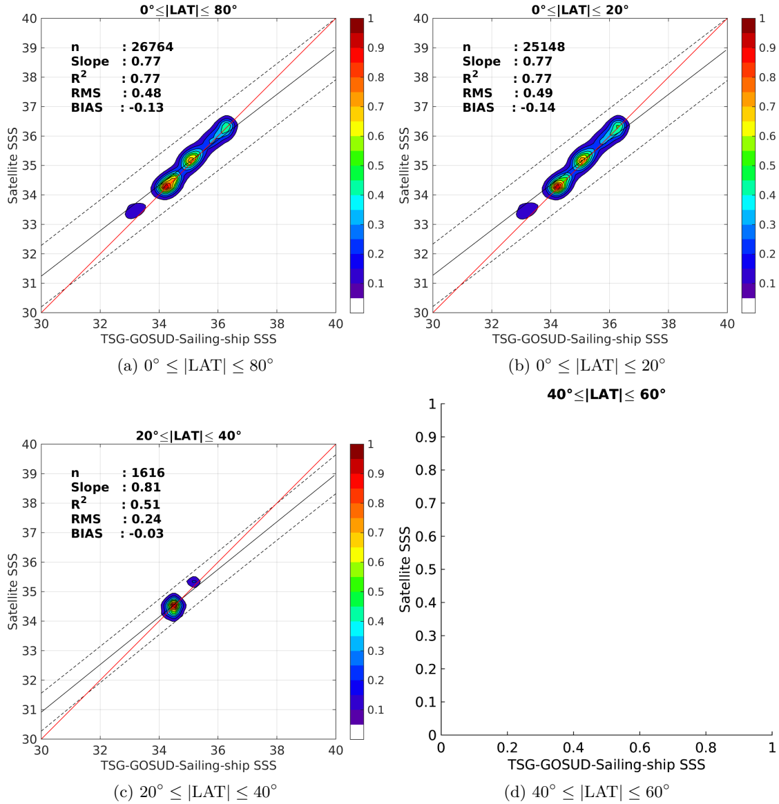
Figure 9: Contour maps of the concentration of SMOS-L3-CATDS-CECOS-LOCEAN-V2-18DAYS-25KM SSS (y-axis) versus TSG-GOSUD-Sailing-ship SSS (x-axis) at match-up pairs for different latitude bands. For each plot, the red line shows x=y . The black thin and dashed lines indicate a linear fit through the data cloud and the \pm 95\% confidence levels, respectively. The number match-up pairs n , the slope and R^2 coefficient of the linear fit, the root mean square (RMS) and the mean bias between satellite and in situ data are indicated for each latitude band in each plots.
