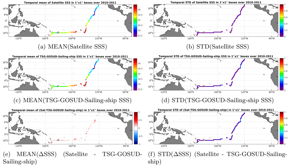
Figure 6: Temporal mean (left) and STD (right) of SSS from SMOS-L3-CATDS-CECOS-LOCEAN-V2-18DAYS-25KM (top), TSG-GOSUD-Sailing-ship (middle), and of \Delta SSS (Satellite - TSG-GOSUD-Sailing-ship). Only match-up pairs are used to generate these maps.
