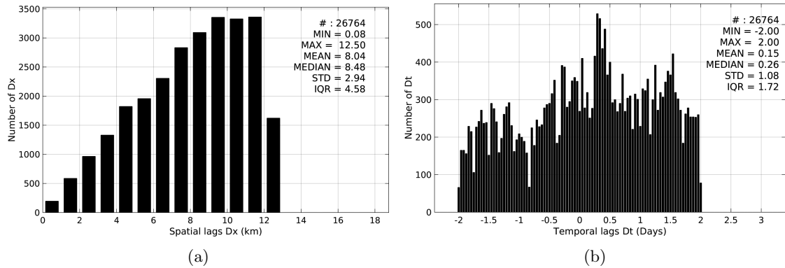
Figure 5: Histograms of the spatial (a) and temporal (b) lags between the time of the TSG-GOSUD-Sailing-ship measurements and the date of the corresponding SMOS-L3-CATDS-CECOS-LOCEAN-V2-18DAYS-25KM SSS product.
