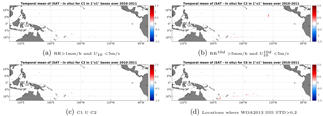
Figure 12: Temporal mean gridded over spatial boxes of size 1^\circ \times 1^\circ of \Delta SSS (SMOS-L3-CATDS-CECOS-LOCEAN-V2-18DAYS-25KM - TSG-GOSUD-Sailing-ship) for 4 different subdatasets corresponding to: RR > 1\text{mm/h} and U_{10} < 5\text{m/s} (a), RR^{10d} > 5\text{mm/h} and U_{10}^{10d} < 5\text{m/s} (b), C1 U C2 (c), Locations where WOA2013 SSS STD > 0.2 (d).
