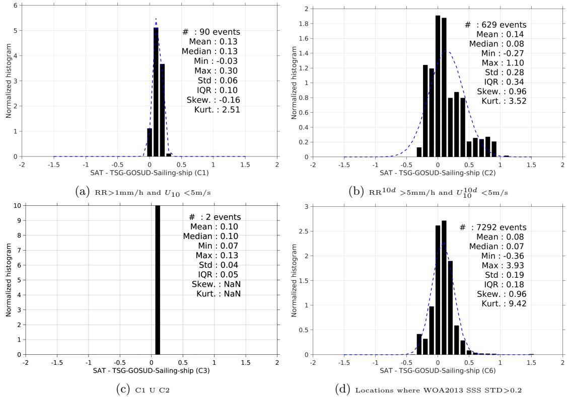
Figure 13: Normalized histogram of \Delta\text{SSS} (SMOS-L3-CATDS-CECOS-LOCEAN-V2-18DAYS-25KM - TSG-GOSUD-Sailing-ship) for 6 different subdatasets corresponding to: RR > 1\text{mm/h} and U_{10} < 5\text{m/s} (a), RR^{10d} > 5\text{mm/h} and U_{10}^{10d} < 5\text{m/s} (b), C1 U C2 (c), Locations where WOA2013 SSS STD > 0.2 (d).
