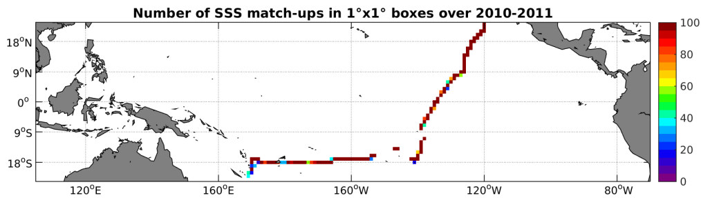
Figure 4: Number of SSS match-ups between TSG-GOSUD-Sailing-ship SSS and the SMOS-L3-CATDS-CECOS-LOCEAN-V2-18DAYS-25KM SSS product for the Tropical Pacific Ocean Pi-MEP region over 1^\circ \times 1^\circ boxes and for the full satellite product period.
