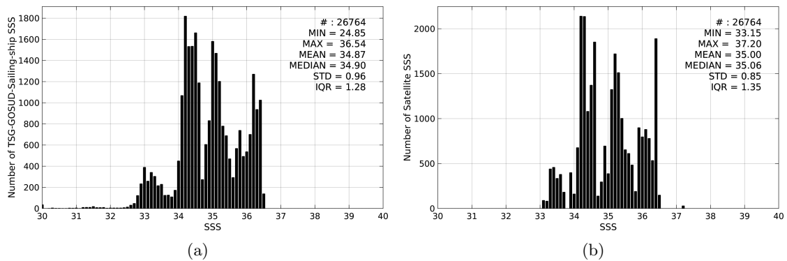
Figure 2: Histograms of SSS from TSG-GOSUD-Sailing-ship (a) and SMOS-L3-CATDS-CECOS-LOCEAN-V2-18DAYS-25KM (b) considering all match-up pairs per bins of 0.1 over the Tropical Pacific Ocean Pi-MEP region and for the full satellite product period.
