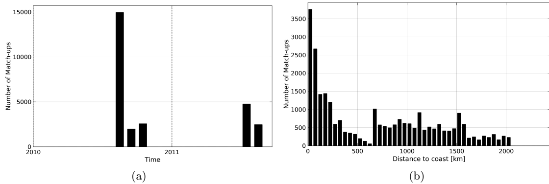
Figure 1: Number of match-ups between TSG-GOSUD-Sailing-ship and SMOS-L3-CATDS-CECOS-LOCEAN-V2-18DAYS-25KM SSS as a function of time (a) and as function of the distance to coast (b) over the Tropical Pacific Ocean Pi-MEP region and for the full satellite product period.
