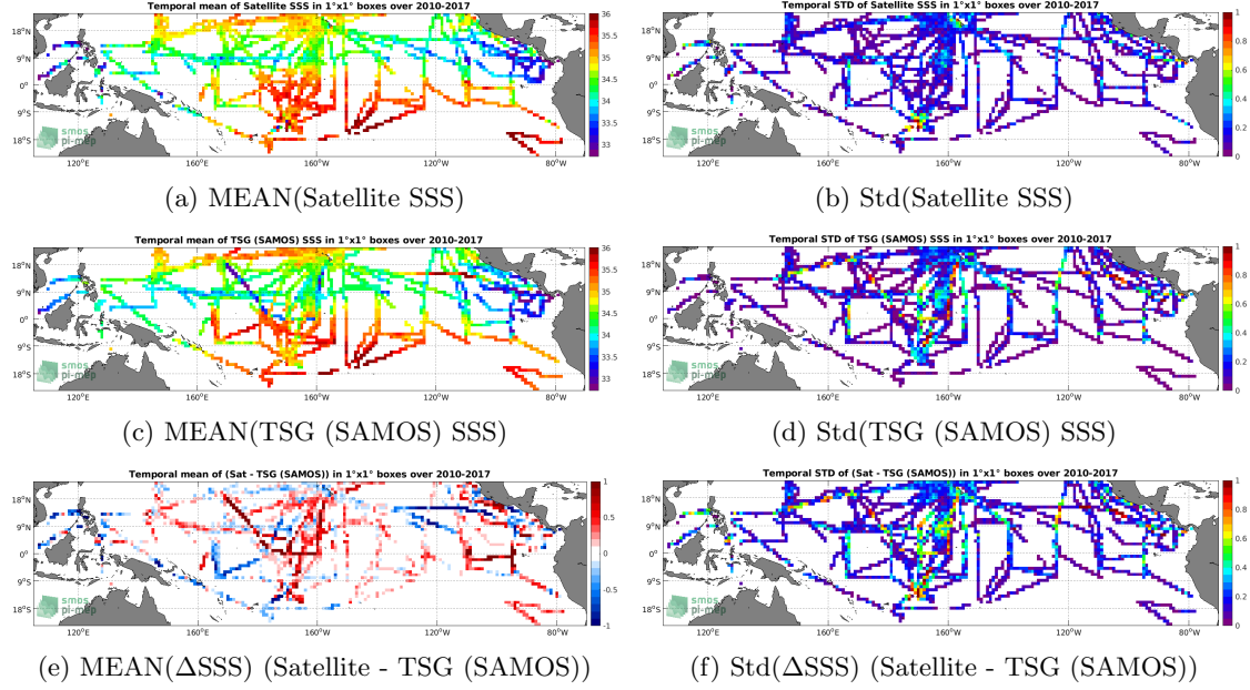
Figure 6: Temporal mean (left) and Std (right) of SSS from SMOS SSS L3 v2 - Monthly - 0.25 Deg (CATDS-CECOS-IFREMER) (top), TSG (SAMOS) (middle), and of \Delta SSS (Satellite - TSG (SAMOS)). Only match-up pairs are used to generate these maps.
