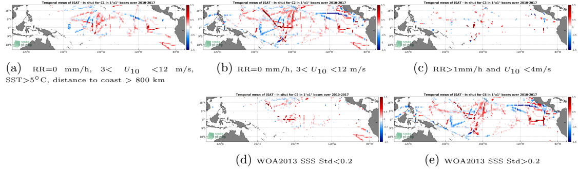
Figure 12: Temporal mean gridded over spatial boxes of size 1^{\circ}\times 1^{\circ} of \Delta\text{SSS} (SMOS SSS L3 v2 - Monthly - 0.25 Deg (CATDS-CECOS-IFREMER) - TSG (SAMOS)) for 5 different subdatasets corresponding to: RR=0 mm/h, 3 < U_{10} < 12 m/s, SST > 5^{\circ}\text{C} , distance to coast > 800 km (a), RR=0 mm/h, 3 < U_{10} < 12 m/s (b), RR > 1 mm/h and U_{10} < 4 m/s (c), WOA2013 SSS Std < 0.2 (d), WOA2013 SSS Std > 0.2 (e).
