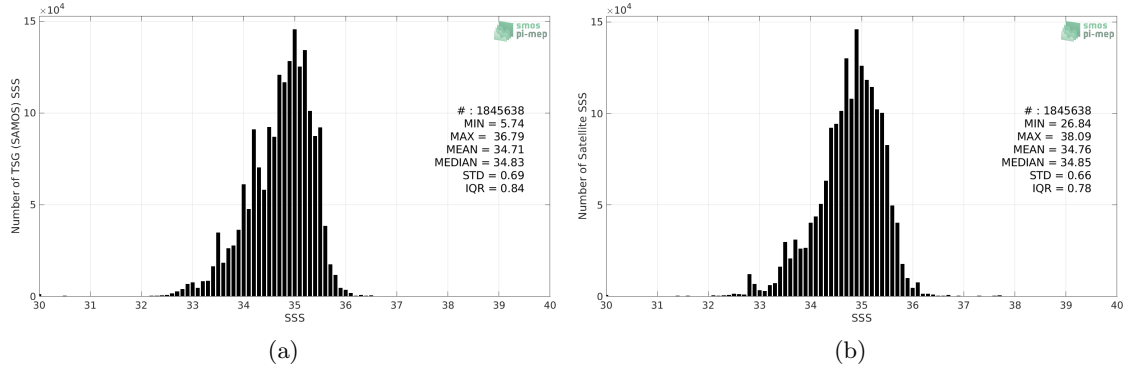
Figure 2: Histograms of SSS from TSG (SAMOS) (a) and SMOS SSS L3 v2 - Monthly - 0.25 Deg (CATDS-CECOS-IFREMER) (b) considering all match-up pairs per bins of 0.1 over the Tropical Pacific Ocean Pi-MEP region and for the full satellite product period.
