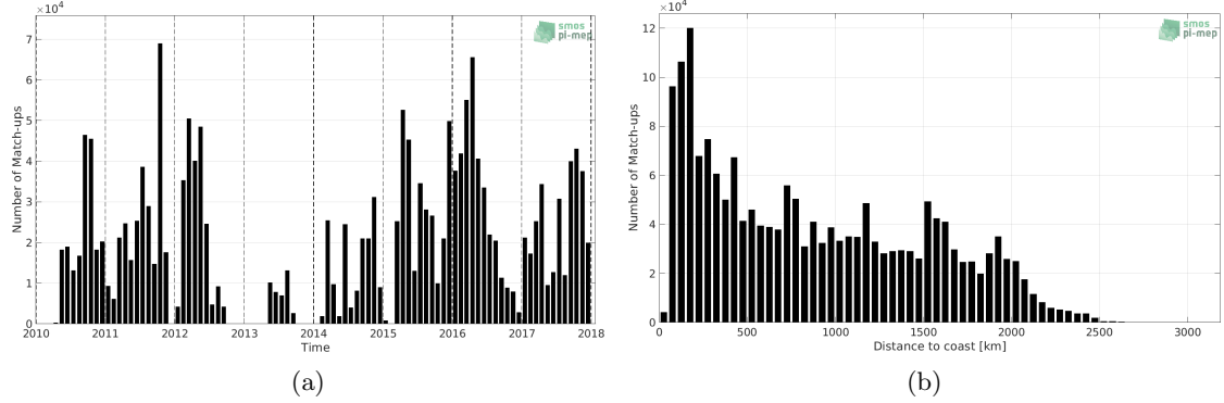
Figure 1: Number of match-ups between TSG (SAMOS) and SMOS SSS L3 v2 - Monthly - 0.25 Deg (CATDS-CECOS-IFREMER) SSS as a function of time (a) and as function of the distance to coast (b) over the Tropical Pacific Ocean Pi-MEP region and for the full satellite product period.
