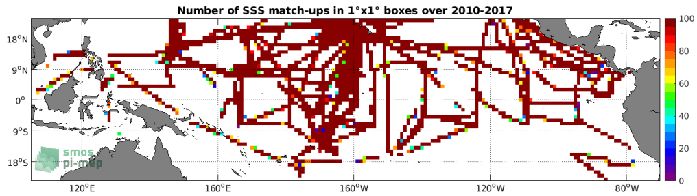
Figure 4: Number of SSS match-ups between TSG (SAMOS) SSS and the SMOS SSS L3 v2 - Monthly - 0.25 Deg (CATDS-CECOS-IFREMER) SSS product for the Tropical Pacific Ocean Pi-MEP region over 1^\circ \times 1^\circ boxes and for the full satellite product period.
