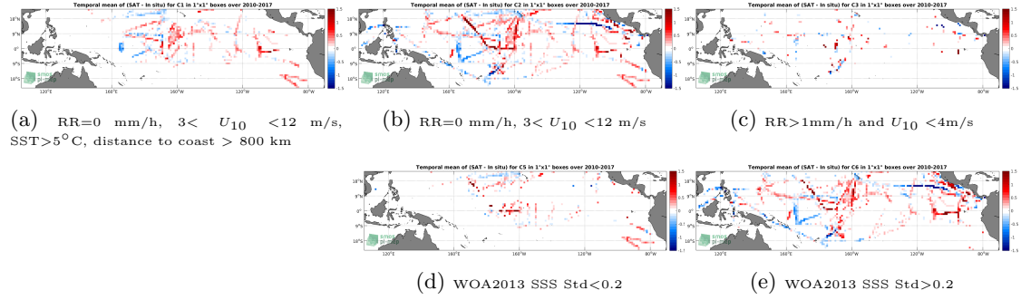
Figure 12: Temporal mean gridded over spatial boxes of size 1^{\circ}\times 1^{\circ} of \Delta\text{SSS} (SMOS SSS L3 v2 - Monthly - 0.25 Deg (CATDS-CECOS-IFREMER) - TSG (SAMOS)) for 5 different subdatasets corresponding to: \text{RR}=0 mm/h, 3 < U_{10} < 12 m/s, \text{SST}>5^{\circ}\text{C} , distance to coast > 800 km (a), \text{RR}=0 mm/h, 3 < U_{10} < 12 m/s (b), \text{RR}>1\text{mm/h} and U_{10} < 4\text{m/s} (c), WOA2013 SSS Std <0.2 (d), WOA2013 SSS Std >0.2 (e).
