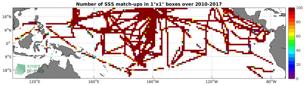
Figure 4: Number of SSS match-ups between TSG (SAMOS) SSS and the SMOS SSS L3 v2 - Monthly - 0.25 Deg (CATDS-CECOS-IFREMER) SSS product for the Tropical Pacific Ocean Pi-MEP region over 1°x1° boxes and for the full satellite product period.
