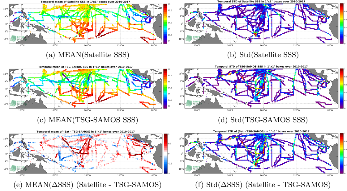
Figure 6: Temporal mean (left) and Std (right) of SSS from SMOS L3 v2 - Monthly - 0.25 Deg (CATDS-CECOS-IFREMER) (top), TSG-SAMOS (middle), and of \Delta SSS (Satellite - TSG-SAMOS). Only match-up pairs are used to generate these maps.
