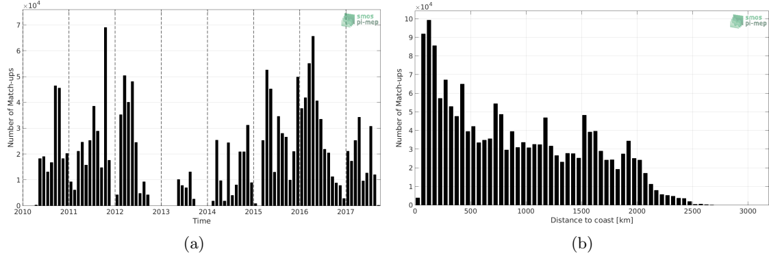
Figure 1: Number of match-ups between TSG-SAMOS and SMOS L3 v2 - Monthly - 0.25 Deg (CATDS-CECOS-IFREMER) SSS as a function of time (a) and as function of the distance to coast (b) over the Tropical Pacific Ocean Pi-MEP region and for the full satellite product period.
