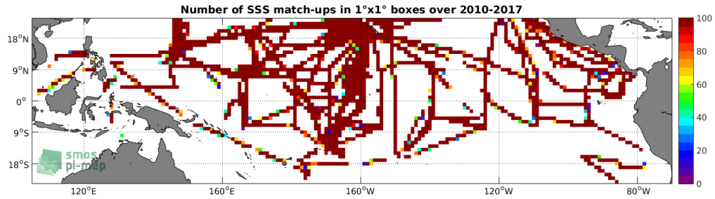
Figure 4: Number of SSS match-ups between TSG-SAMOS SSS and the SMOS L3 v2 - Monthly - 0.25 Deg (CATDS-CECOS-IFREMER) SSS product for the Tropical Pacific Ocean Pi-MEP region over 1°x1° boxes and for the full satellite product period.
