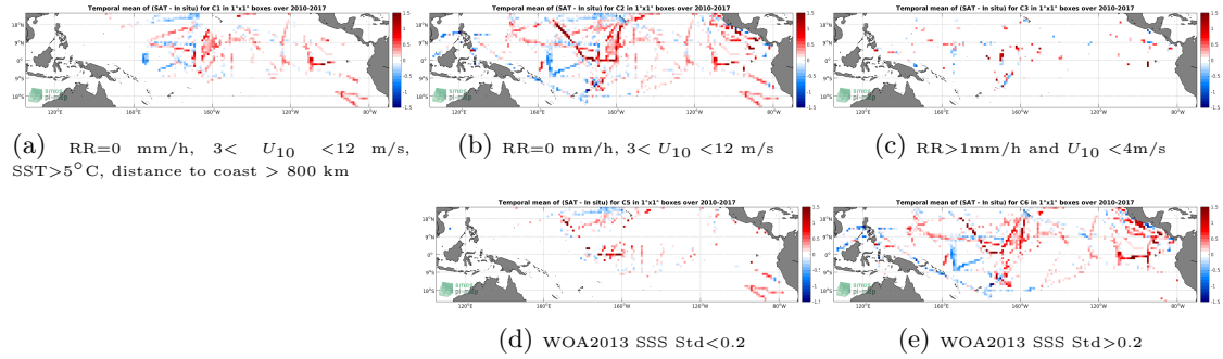
Figure 12: Temporal mean gridded over spatial boxes of size 1^{\circ}\times 1^{\circ} of \Delta\text{SSS} (SMOS L3 v2 - Monthly - 0.25^{\circ} Deg (CATDS-CECOS-IFREMER) - TSG-SAMOS) for 5 different subdatasets corresponding to: RR=0 mm/h, 3 < U_{10} < 12 m/s, SST > 5^{\circ}\text{C} , distance to coast > 800 km (a), RR=0 mm/h, 3 < U_{10} < 12 m/s (b), RR > 1 mm/h and U_{10} < 4 m/s (c), WOA2013 SSS Std < 0.2 (d), WOA2013 SSS Std > 0.2 (e).
