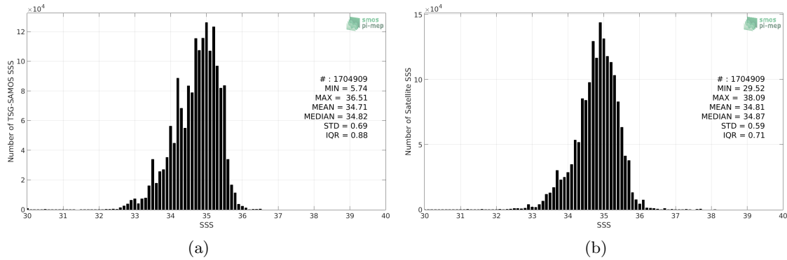
Figure 2: Histograms of SSS from TSG-SAMOS (a) and SMOS L3 v2 - Monthly - 0.25 Deg (CATDS-CECOS-IFREMER) (b) considering all match-up pairs per bins of 0.1 over the Tropical Pacific Ocean Pi-MEP region and for the full satellite product period.
