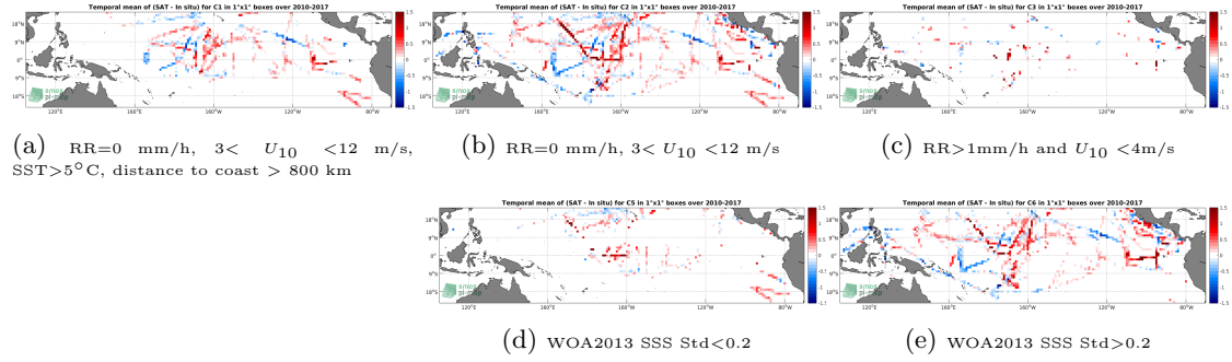
Figure 12: Temporal mean gridded over spatial boxes of size 1^\circ \times 1^\circ of \Delta SSS (SMOS-L3-CATDS-IFREMER-CECOS-V2-MONTHLY-0.25DEG - TSG-SAMOS) for 5 different subdatasets corresponding to: RR=0 mm/h, 3 < U_{10} < 12 m/s, SST > 5^\circ C , distance to coast > 800 km (a), RR=0 mm/h, 3 < U_{10} < 12 m/s (b), RR > 1 mm/h and U_{10} < 4 m/s (c), WOA2013 SSS Std < 0.2 (d), WOA2013 SSS Std > 0.2 (e).
