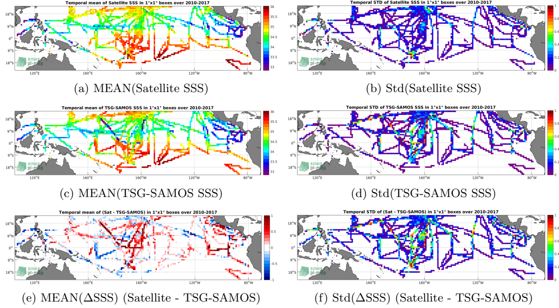
Figure 6: Temporal mean (left) and Std (right) of SSS from SMOS-L3-CATDS-IFREMER-CECOS-V2-MONTHLY-0.25DEG (top), TSG-SAMOS (middle), and of \Delta SSS (Satellite - TSG-SAMOS). Only match-up pairs are used to generate these maps.
