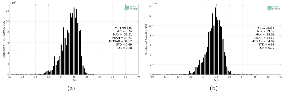
Figure 2: Histograms of SSS from TSG-SAMOS (a) and SMOS-L3-CATDS-IFREMER-CECOS-V2-MONTHLY-0.25DEG (b) considering all match-up pairs per bins of 0.1 over the Tropical Pacific Ocean Pi-MEP region and for the full satellite product period.
