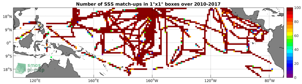
Figure 4: Number of SSS match-ups between TSG-SAMOS SSS and the SMOS-L3-CATDS-IFREMER-CECOS-V2-MONTHLY-0.25DEG SSS product for the Tropical Pacific Ocean Pi-MEP region over 1°x1° boxes and for the full satellite product period.
