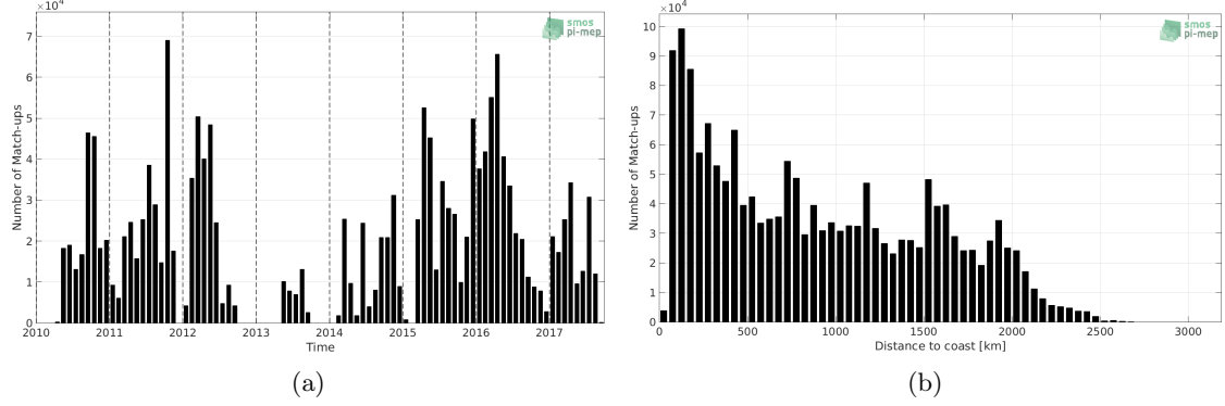
Figure 1: Number of match-ups between TSG-SAMOS and SMOS-L3-CATDS-IFREMER-CECOS-V2-MONTHLY-0.25DEG SSS as a function of time (a) and as function of the distance to coast (b) over the Tropical Pacific Ocean Pi-MEP region and for the full satellite product period.
