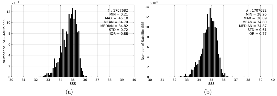
Figure 2: Histograms of SSS from TSG-SAMOS (a) and SMOS-L3-CATDS-IFREMER-CECOS-V2-MONTHLY-0.25DEG (b) considering all match-up pairs per bins of 0.1 over the Tropical Pacific Ocean Pi-MEP region and for the full satellite product period.
