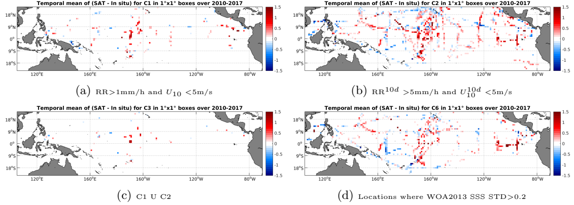
Figure 12: Temporal mean gridded over spatial boxes of size 1^\circ \times 1^\circ of \Delta SSS (SMOS-L3-CATDS-IFREMER-CECOS-V2-MONTHLY-0.25DEG - TSG-SAMOS) for 4 different subdatasets corresponding to: RR > 1\text{mm/h} and U_{10} < 5\text{m/s} (a), RR^{10d} > 5\text{mm/h} and U_{10}^{10d} < 5\text{m/s} (b), C1 U C2 (c), Locations where WOA2013 SSS STD > 0.2 (d).
