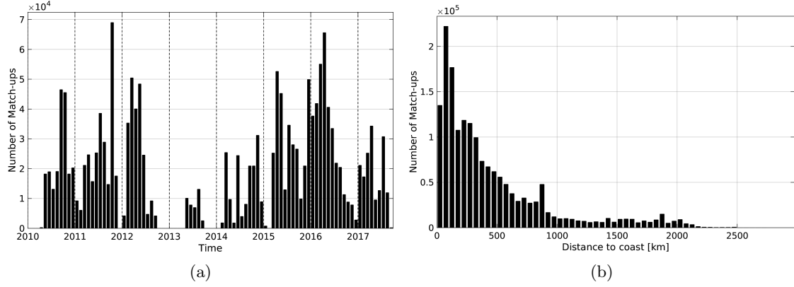
Figure 1: Number of match-ups between TSG-SAMOS and SMOS-L3-CATDS-IFREMER-CECOS-V2-MONTHLY-0.25DEG SSS as a function of time (a) and as function of the distance to coast (b) over the Tropical Pacific Ocean Pi-MEP region and for the full satellite product period.
