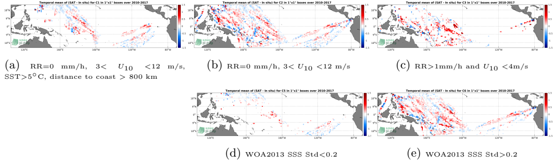
Figure 12: Temporal mean gridded over spatial boxes of size 1^{\circ}\times 1^{\circ} of \Delta\text{SSS} (SMOS SSS L3 v2 - Monthly - 0.25 Deg (CATDS-CECOS-IFREMER) - TSG (LEGOS-DM)) for 5 different subdatasets corresponding to: RR=0 mm/h, 3 < U_{10} < 12 m/s, SST > 5^{\circ}\text{C} , distance to coast > 800 km (a), RR=0 mm/h, 3 < U_{10} < 12 m/s (b), RR > 1 mm/h and U_{10} < 4 m/s (c), WOA2013 SSS Std < 0.2 (d), WOA2013 SSS Std > 0.2 (e).
