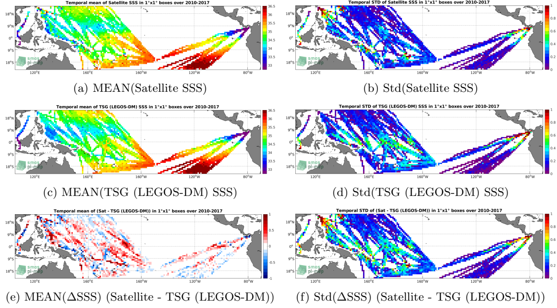
Figure 6: Temporal mean (left) and Std (right) of SSS from SMOS SSS L3 v2 - Monthly - 0.25 Deg (CATDS-CECOS-IFREMER) (top), TSG (LEGOS-DM) (middle), and of \Delta SSS (Satellite - TSG (LEGOS-DM)). Only match-up pairs are used to generate these maps.
