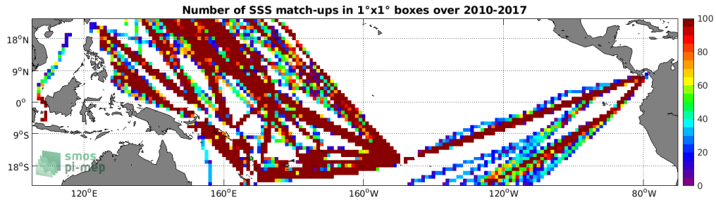
Figure 4: Number of SSS match-ups between TSG (LEGOS-DM) SSS and the SMOS SSS L3 v2 - Monthly - 0.25 Deg (CATDS-CECOS-IFREMER) SSS product for the Tropical Pacific Ocean Pi-MEP region over 1^\circ \times 1^\circ boxes and for the full satellite product period.
