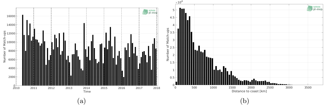
Figure 1: Number of match-ups between TSG (LEGOS-DM) and SMOS SSS L3 v2 - Monthly - 0.25 Deg (CATDS-CECOS-IFREMER) SSS as a function of time (a) and as function of the distance to coast (b) over the Tropical Pacific Ocean Pi-MEP region and for the full satellite product period.
