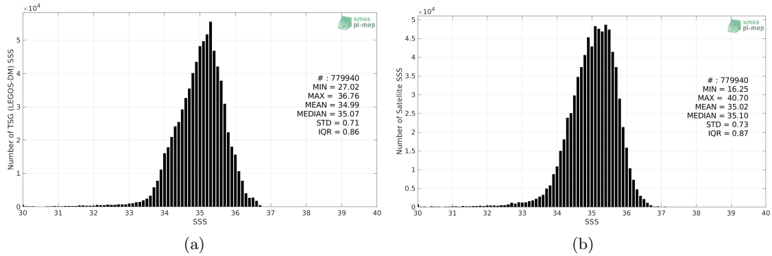
Figure 2: Histograms of SSS from TSG (LEGOS-DM) (a) and SMOS SSS L3 v2 - Monthly - 0.25 Deg (CATDS-CECOS-IFREMER) (b) considering all match-up pairs per bins of 0.1 over the Tropical Pacific Ocean Pi-MEP region and for the full satellite product period.
