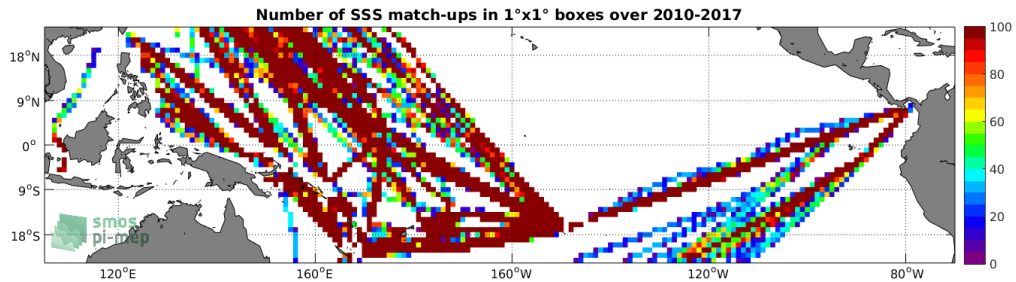
Figure 4: Number of SSS match-ups between TSG (LEGOS-DM) SSS and the SMOS SSS L3 v2 - Monthly - 0.25 Deg (CATDS-CECOS-IFREMER) SSS product for the Tropical Pacific Ocean Pi-MEP region over 1^\circ \times 1^\circ boxes and for the full satellite product period.
