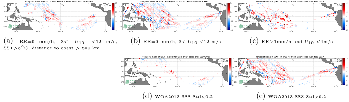
Figure 12: Temporal mean gridded over spatial boxes of size 1^{\circ}\times 1^{\circ} of \Delta\text{SSS} (SMOS SSS L3 v2 - Monthly - 0.25 Deg (CATDS-CECOS-IFREMER) - TSG (LEGOS-DM)) for 5 different subdatasets corresponding to: \text{RR}=0 mm/h, 3 < U_{10} < 12 m/s, \text{SST}>5^{\circ}\text{C} , distance to coast > 800 km (a), \text{RR}=0 mm/h, 3 < U_{10} < 12 m/s (b), \text{RR}>1\text{mm/h} and U_{10} < 4\text{m/s} (c), WOA2013 SSS Std <0.2 (d), WOA2013 SSS Std >0.2 (e).
