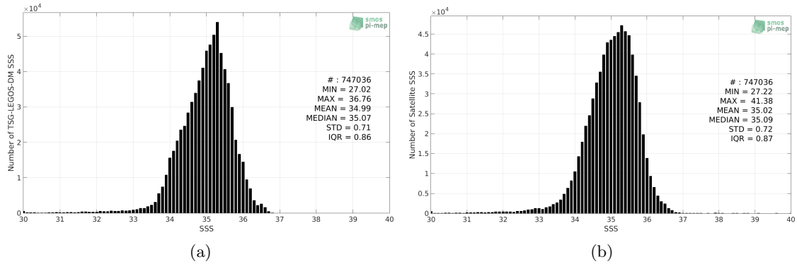
Figure 2: Histograms of SSS from TSG-LEGOS-DM (a) and SMOS L3 v2 - Monthly - 0.25 Deg (CATDS-CECOS-IFREMER) (b) considering all match-up pairs per bins of 0.1 over the Tropical Pacific Ocean Pi-MEP region and for the full satellite product period.
