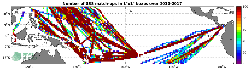
Figure 4: Number of SSS match-ups between TSG-LEGOS-DM SSS and the SMOS L3 v2 - Monthly - 0.25 Deg (CATDS-CECOS-IFREMER) SSS product for the Tropical Pacific Ocean Pi-MEP region over 1°x1° boxes and for the full satellite product period.
