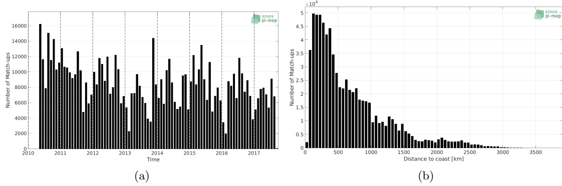
Figure 1: Number of match-ups between TSG-LEGOS-DM and SMOS L3 v2 - Monthly - 0.25 Deg (CATDS-CECOS-IFREMER) SSS as a function of time (a) and as function of the distance to coast (b) over the Tropical Pacific Ocean Pi-MEP region and for the full satellite product period.
