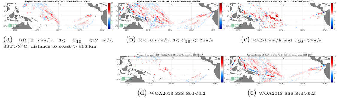
Figure 12: Temporal mean gridded over spatial boxes of size 1^{\circ}\times 1^{\circ} of \Delta\text{SSS} (SMOS L3 v2 - Monthly - 0.25 Deg (CATDS-CECOS-IFREMER) - TSG-LEGOS-DM) for 5 different subdatasets corresponding to: RR=0 mm/h, 3 < U_{10} < 12 m/s, SST > 5^{\circ}\text{C} , distance to coast > 800 km (a), RR=0 mm/h, 3 < U_{10} < 12 m/s (b), RR > 1 mm/h and U_{10} < 4 m/s (c), WOA2013 SSS Std < 0.2 (d), WOA2013 SSS Std > 0.2 (e).
