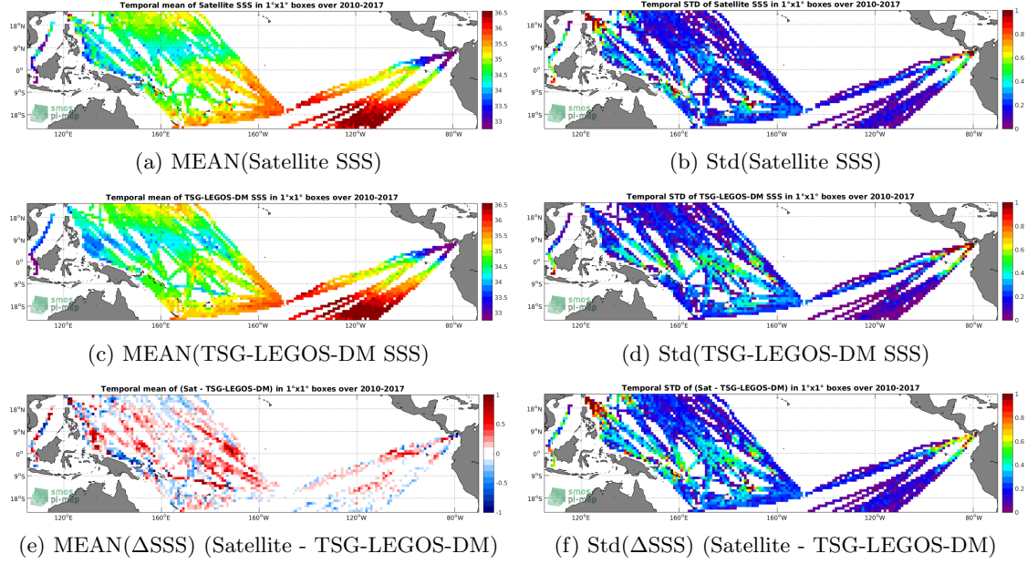
Figure 6: Temporal mean (left) and Std (right) of SSS from SMOS L3 v2 - Monthly - 0.25 Deg (CATDS-CECOS-IFREMER) (top), TSG-LEGOS-DM (middle), and of \Delta SSS (Satellite - TSG-LEGOS-DM). Only match-up pairs are used to generate these maps.
