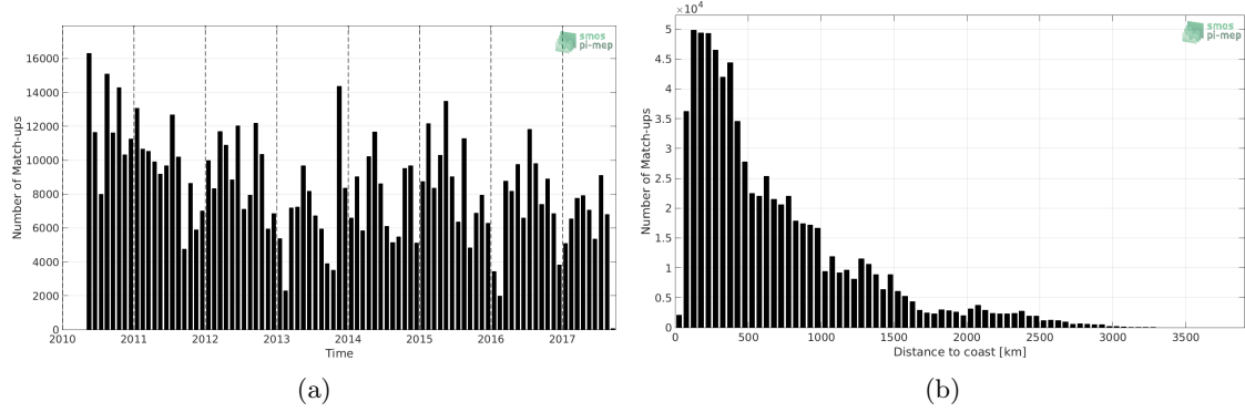
Figure 1: Number of match-ups between TSG-LEGOS-DM and SMOS-L3-CATDS-IFREMER-CECOS-V2-MONTHLY-0.25DEG SSS as a function of time (a) and as function of the distance to coast (b) over the Tropical Pacific Ocean Pi-MEP region and for the full satellite product period.
