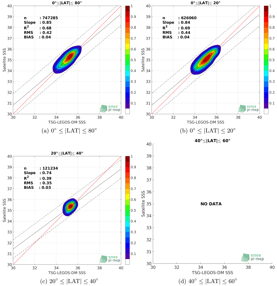
Figure 9: Contour maps of the concentration of SMOS-L3-CATDS-IFREMER-CECOS-V2-MONTHLY-0.25DEG SSS (y-axis) versus TSG-LEGOS-DM SSS (x-axis) at match-up pairs for different latitude bands. For each plot, the red line shows x=y . The black thin and dashed lines indicate a linear fit through the data cloud and the \pm 95\% confidence levels, respectively. The number match-up pairs n , the slope and R^2 coefficient of the linear fit, the root mean square (RMS) and the mean bias between satellite and in situ data are indicated for each latitude band in each plots.
