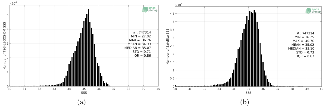
Figure 2: Histograms of SSS from TSG-LEGOS-DM (a) and SMOS-L3-CATDS-IFREMER-CECOS-V2-MONTHLY-0.25DEG (b) considering all match-up pairs per bins of 0.1 over the Tropical Pacific Ocean Pi-MEP region and for the full satellite product period.
