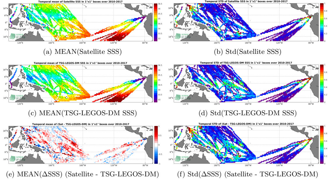
Figure 6: Temporal mean (left) and Std (right) of SSS from SMOS-L3-CATDS-IFREMER-CECOS-V2-MONTHLY-0.25DEG (top), TSG-LEGOS-DM (middle), and of \Delta SSS (Satellite - TSG-LEGOS-DM). Only match-up pairs are used to generate these maps.
