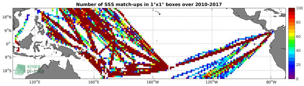
Figure 4: Number of SSS match-ups between TSG-LEGOS-DM SSS and the SMOS-L3-CATDS-IFREMER-CECOS-V2-MONTHLY-0.25DEG SSS product for the Tropical Pacific Ocean Pi-MEP region over 1^\circ \times 1^\circ boxes and for the full satellite product period.
