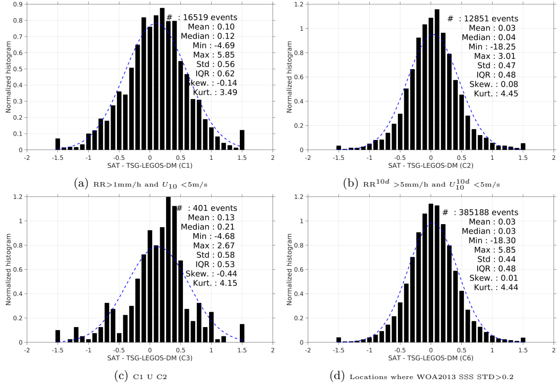
Figure 13: Normalized histogram of \Delta SSS (SMOS-L3-CATDS-IFREMER-CECOS-V2-MONTHLY-0.25DEG - TSG-LEGOS-DM) for 6 different subdatasets corresponding to: RR>1mm/h and U_{10} < 5\text{m/s} (a), RR^{10d} > 5\text{mm/h} and U_{10}^{10d} < 5\text{m/s} (b), C1 U C2 (c), Locations where WOA2013 SSS STD>0.2 (d).
