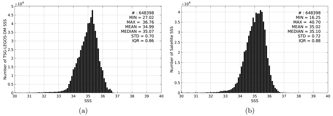
Figure 2: Histograms of SSS from TSG-LEGOS-DM (a) and SMOS-L3-CATDS-IFREMER-CECOS-V2-MONTHLY-0.25DEG (b) considering all match-up pairs per bins of 0.1 over the Tropical Pacific Ocean Pi-MEP region and for the full satellite product period.
