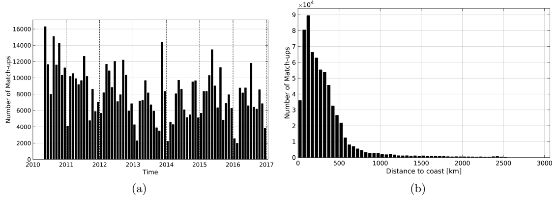
Figure 1: Number of match-ups between TSG-LEGOS-DM and SMOS-L3-CATDS-IFREMER-CECOS-V2-MONTHLY-0.25DEG SSS as a function of time (a) and as function of the distance to coast (b) over the Tropical Pacific Ocean Pi-MEP region and for the full satellite product period.
