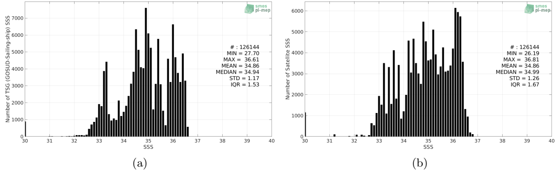
Figure 2: Histograms of SSS from TSG (GOSUD-Sailing-ship) (a) and SMOS SSS L3 v2 - Monthly - 0.25 Deg (CATDS-CECOS-IFREMER) (b) considering all match-up pairs per bins of 0.1 over the Tropical Pacific Ocean Pi-MEP region and for the full satellite product period.
