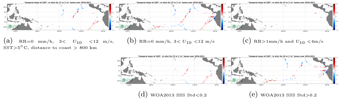
Figure 12: Temporal mean gridded over spatial boxes of size 1^\circ \times 1^\circ of \Delta SSS (SMOS SSS L3 v2 - Monthly - 0.25 Deg (CATDS-CECOS-IFREMER) - TSG (GOSUD-Sailing-ship)) for 5 different subdatasets corresponding to: RR=0 mm/h, 3 < U_{10} < 12 m/s, SST >5^\circ\text{C} , distance to coast > 800 km (a), RR=0 mm/h, 3 < U_{10} < 12 m/s (b), RR >1 mm/h and U_{10} < 4 m/s (c), WOA2013 SSS Std <0.2 (d), WOA2013 SSS Std >0.2 (e).
