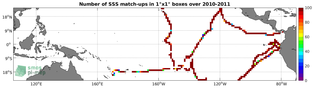
Figure 4: Number of SSS match-ups between TSG (GOSUD-Sailing-ship) SSS and the SMOS SSS L3 v2 - Monthly - 0.25 Deg (CATDS-CECOS-IFREMER) SSS product for the Tropical Pacific Ocean Pi-MEP region over 1^\circ \times 1^\circ boxes and for the full satellite product period.
