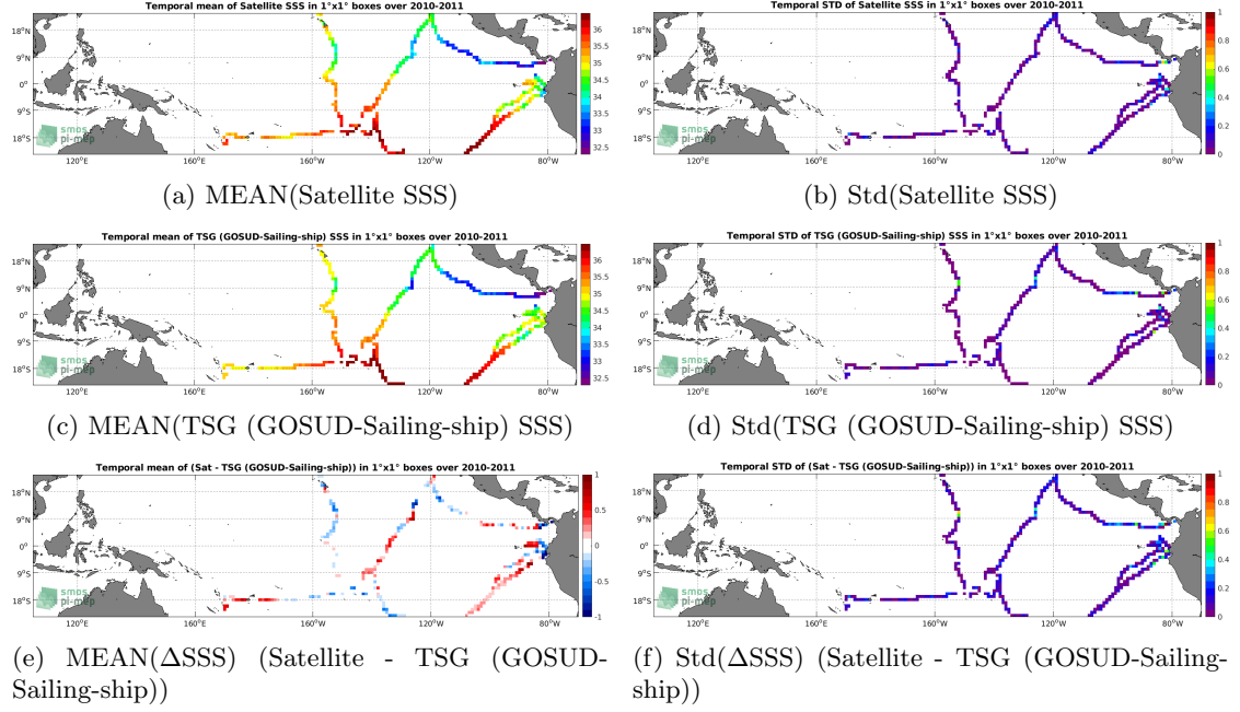
Figure 6: Temporal mean (left) and Std (right) of SSS from SMOS SSS L3 v2 - Monthly - 0.25 Deg (CATDS-CECOS-IFREMER) (top), TSG (GOSUD-Sailing-ship) (middle), and of \Delta SSS (Satellite - TSG (GOSUD-Sailing-ship)). Only match-up pairs are used to generate these maps.
