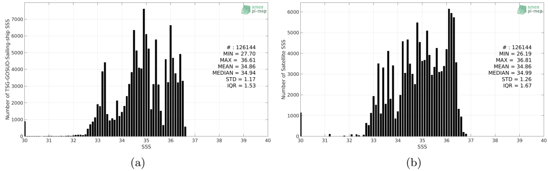
Figure 2: Histograms of SSS from TSG-GOSUD-Sailing-ship (a) and SMOS-L3-CATDS-IFREMER-CECOS-V2-MONTHLY-0.25DEG (b) considering all match-up pairs per bins of 0.1 over the Tropical Pacific Ocean Pi-MEP region and for the full satellite product period.
