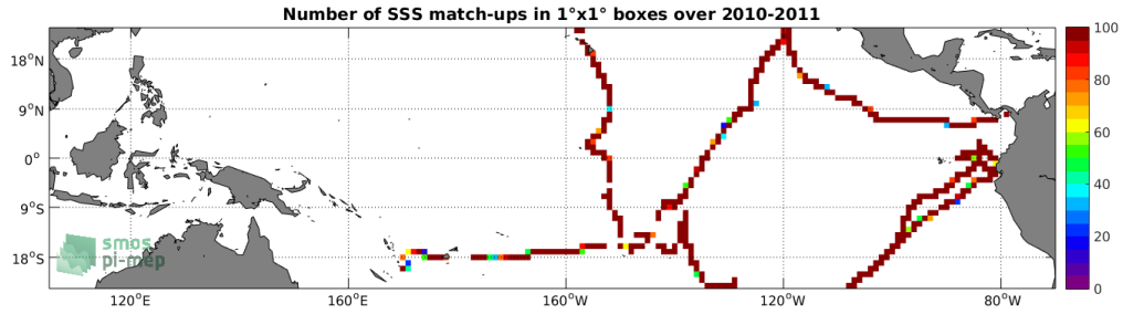
Figure 4: Number of SSS match-ups between TSG-GOSUD-Sailing-ship SSS and the SMOS-L3-CATDS-IFREMER-CECOS-V2-MONTHLY-0.25DEG SSS product for the Tropical Pacific Ocean Pi-MEP region over 1^\circ \times 1^\circ boxes and for the full satellite product period.
