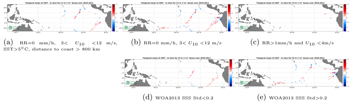
Figure 12: Temporal mean gridded over spatial boxes of size 1^\circ \times 1^\circ of \Delta SSS (SMOS-L3-CATDS-IFREMER-CECOS-V2-MONTHLY-0.25DEG - TSG-GOSUD-Sailing-ship) for 5 different sub-datasets corresponding to: RR=0 mm/h, 3 < U_{10} < 12 m/s, SST > 5^\circ C , distance to coast > 800 km (a), RR=0 mm/h, 3 < U_{10} < 12 m/s (b), RR > 1 mm/h and U_{10} < 4 m/s (c), WOA2013 SSS Std < 0.2 (d), WOA2013 SSS Std > 0.2 (e).
