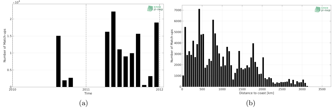
Figure 1: Number of match-ups between TSG-GOSUD-Sailing-ship and SMOS-L3-CATDS-IFREMER-CECOS-V2-MONTHLY-0.25DEG SSS as a function of time (a) and as function of the distance to coast (b) over the Tropical Pacific Ocean Pi-MEP region and for the full satellite product period.
