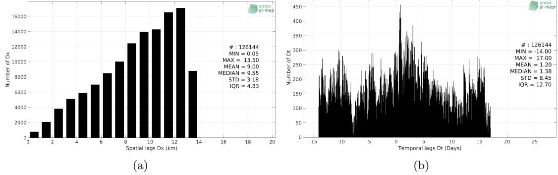
Figure 5: Histograms of the spatial (a) and temporal (b) lags between the time of the TSG-GOSUD-Sailing-ship measurements and the date of the corresponding SMOS-L3-CATDS-IFREMER-CECOS-V2-MONTHLY-0.25DEG SSS product.
