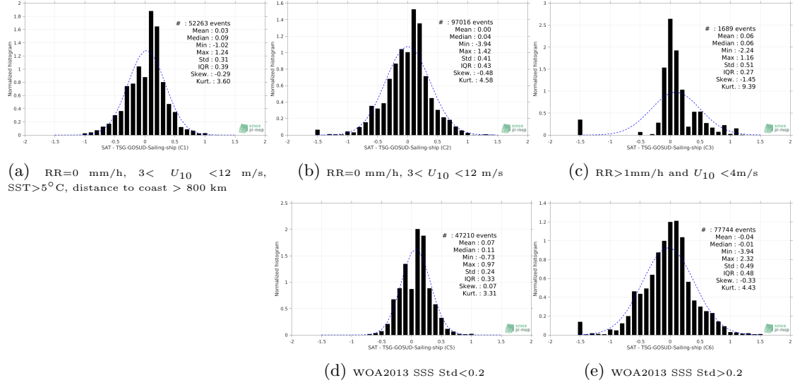
Figure 13: Normalized histogram of \Delta SSS (SMOS-L3-CATDS-IFREMER-CECOS-V2-MONTHLY-0.25DEG - TSG-GOSUD-Sailing-ship) for 5 different subdatasets corresponding to: RR=0 mm/h, 3 < U_{10} < 12 m/s, SST>5°C, distance to coast > 800 km (a), RR=0 mm/h, 3 < U_{10} < 12 m/s (b), RR>1mm/h and U_{10} < 4 m/s (c), WOA2013 SSS Std<0.2 (d), WOA2013 SSS Std>0.2 (e).
