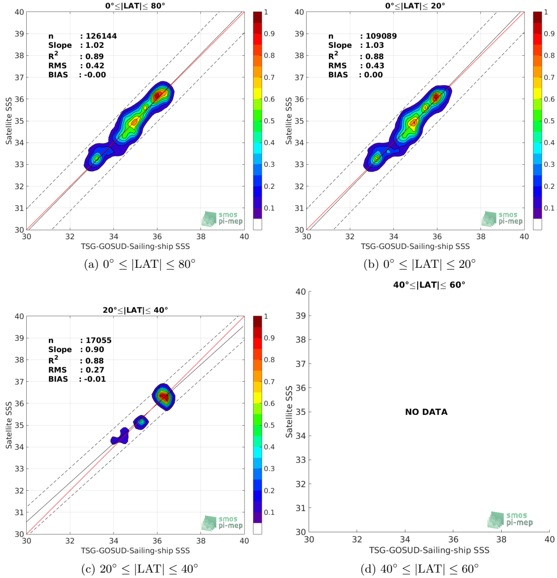
Figure 9: Contour maps of the concentration of SMOS-L3-CATDS-IFREMER-CECOS-V2-MONTHLY-0.25DEG SSS (y-axis) versus TSG-GOSUD-Sailing-ship SSS (x-axis) at match-up pairs for different latitude bands. For each plot, the red line shows x=y . The black thin and dashed lines indicate a linear fit through the data cloud and the \pm 95\% confidence levels, respectively. The number match-up pairs n , the slope and R^2 coefficient of the linear fit, the root mean square (RMS) and the mean bias between satellite and in situ data are indicated for each latitude band in each plots.
