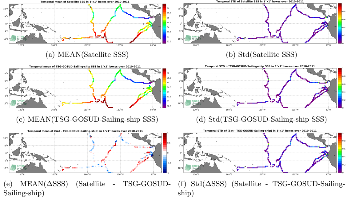
Figure 6: Temporal mean (left) and Std (right) of SSS from SMOS-L3-CATDS-IFREMER-CECOS-V2-MONTHLY-0.25DEG (top), TSG-GOSUD-Sailing-ship (middle), and of \Delta SSS (Satellite - TSG-GOSUD-Sailing-ship). Only match-up pairs are used to generate these maps.
