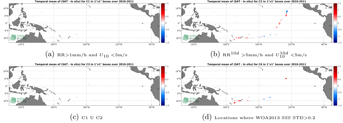
Figure 12: Temporal mean gridded over spatial boxes of size 1^\circ \times 1^\circ of \Delta SSS (SMOS-L3-CATDS-IFREMER-CECOS-V2-MONTHLY-0.25DEG - TSG-GOSUD-Sailing-ship) for 4 different sub-datasets corresponding to: RR > 1mm/h and U_{10} < 5\text{m/s} (a), RR^{10d} > 5\text{mm/h} and U_{10}^{10d} < 5\text{m/s} (b), C1 U C2 (c), Locations where WOA2013 SSS STD > 0.2 (d).
