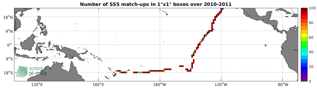
Figure 4: Number of SSS match-ups between TSG-GOSUD-Sailing-ship SSS and the SMOS-L3-CATDS-IFREMER-CECOS-V2-MONTHLY-0.25DEG SSS product for the Tropical Pacific Ocean Pi-MEP region over 1^\circ \times 1^\circ boxes and for the full satellite product period.
