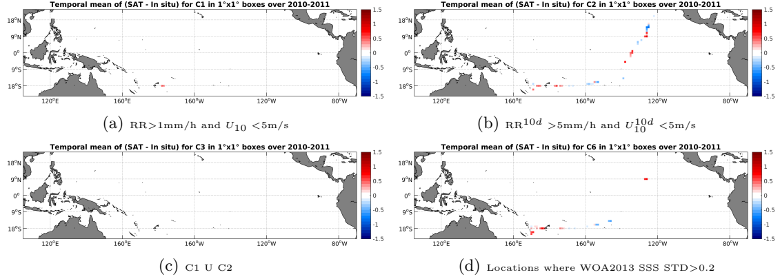
Figure 12: Temporal mean gridded over spatial boxes of size 1^\circ \times 1^\circ of \Delta SSS (SMOS-L3-CATDS-IFREMER-CECOS-V2-MONTHLY-0.25DEG - TSG-GOSUD-Sailing-ship) for 4 different sub-datasets corresponding to: RR > 1\text{mm/h} and U_{10} < 5\text{m/s} (a), RR^{10d} > 5\text{mm/h} and U_{10}^{10d} < 5\text{m/s} (b), C1 U C2 (c), Locations where WOA2013 SSS STD > 0.2 (d).
