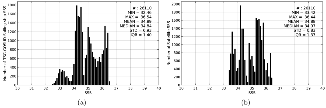
Figure 2: Histograms of SSS from TSG-GOSUD-Sailing-ship (a) and SMOS-L3-CATDS-IFREMER-CECOS-V2-MONTHLY-0.25DEG (b) considering all match-up pairs per bins of 0.1 over the Tropical Pacific Ocean Pi-MEP region and for the full satellite product period.
