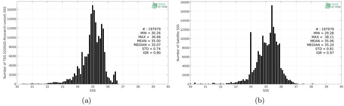
Figure 2: Histograms of SSS from TSG (GOSUD-Research-vessel) (a) and SMOS SSS L3 v2 - Monthly - 0.25 Deg (CATDS-CECOS-IFREMER) (b) considering all match-up pairs per bins of 0.1 over the Tropical Pacific Ocean Pi-MEP region and for the full satellite product period.
