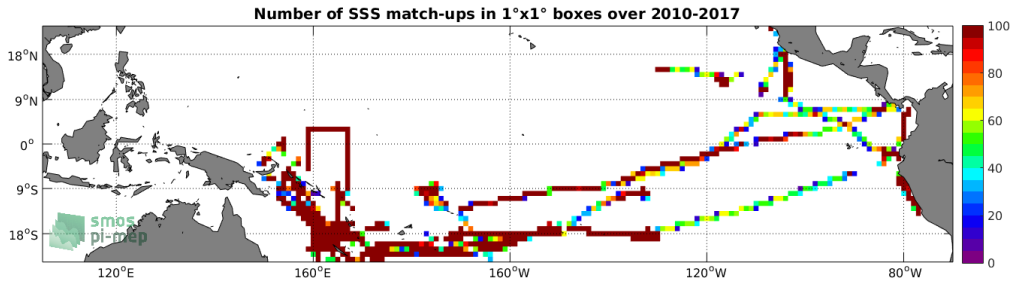
Figure 4: Number of SSS match-ups between TSG (GOSUD-Research-vessel) SSS and the SMOS SSS L3 v2 - Monthly - 0.25 Deg (CATDS-CECOS-IFREMER) SSS product for the Tropical Pacific Ocean Pi-MEP region over 1^\circ \times 1^\circ boxes and for the full satellite product period.
