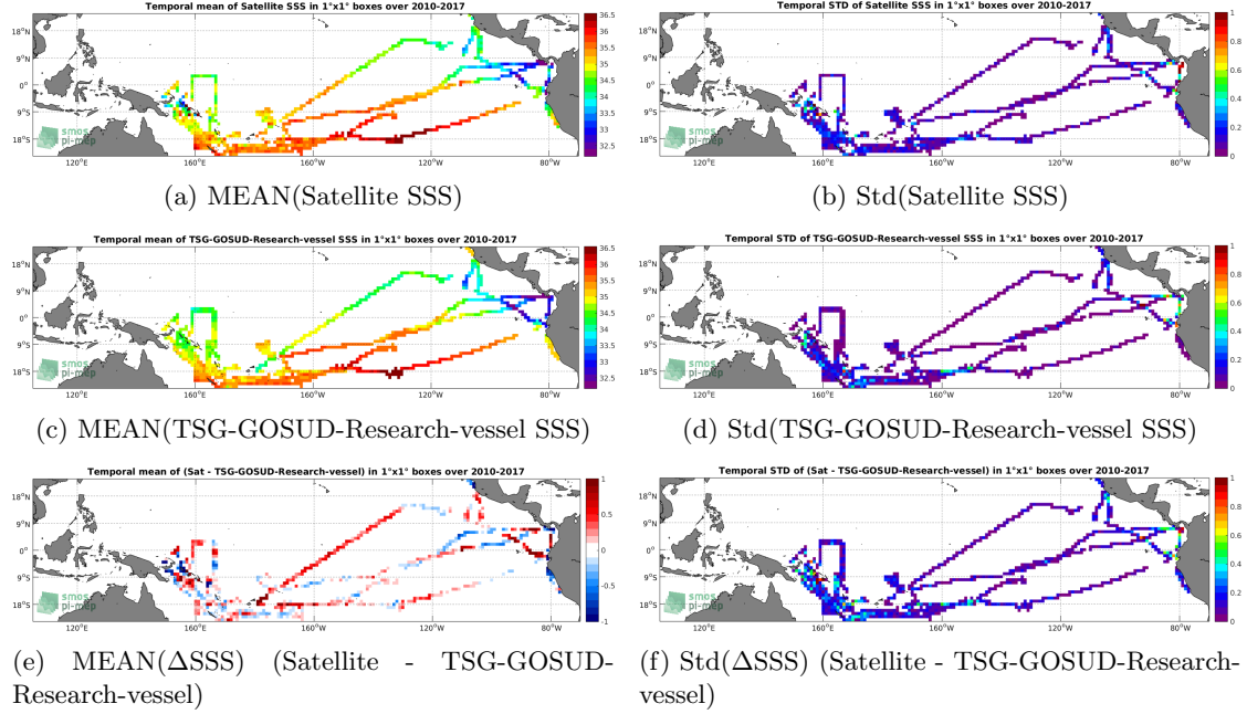
Figure 6: Temporal mean (left) and Std (right) of SSS from SMOS L3 v2 - Monthly - 0.25 Deg (CATDS-CECOS-IFREMER) (top), TSG-GOSUD-Research-vessel (middle), and of \Delta SSS (Satellite - TSG-GOSUD-Research-vessel). Only match-up pairs are used to generate these maps.
