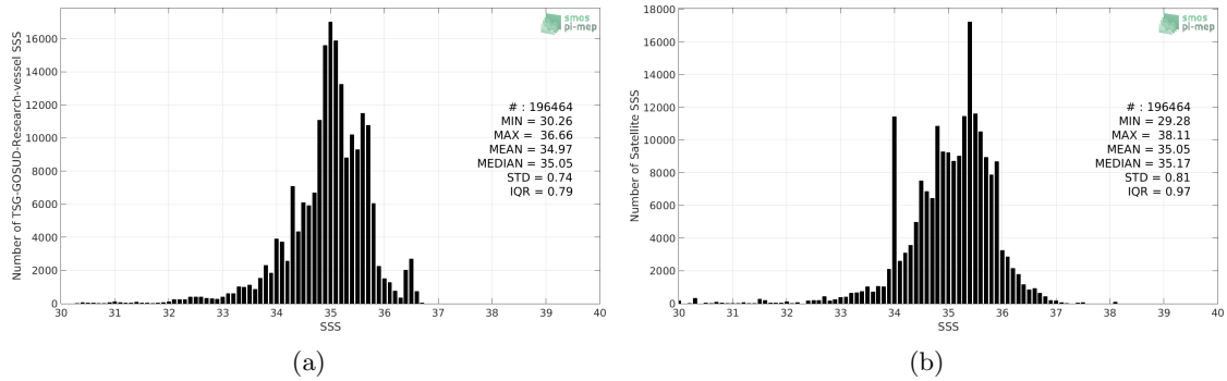
Figure 2: Histograms of SSS from TSG-GOSUD-Research-vessel (a) and SMOS L3 v2 - Monthly - 0.25 Deg (CATDS-CECOS-IFREMER) (b) considering all match-up pairs per bins of 0.1 over the Tropical Pacific Ocean Pi-MEP region and for the full satellite product period.
