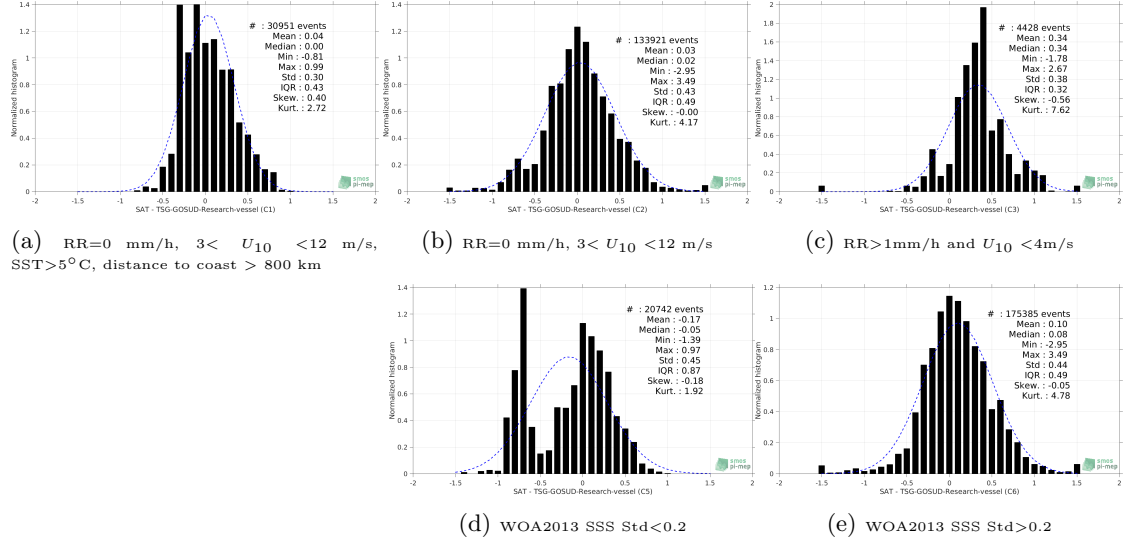
Figure 13: Normalized histogram of \Delta\text{SSS} (SMOS L3 v2 - Monthly - 0.25 Deg (CATDS-CECOS-IFREMER) - TSG-GOSUD-Research-vessel) for 5 different subdatasets corresponding to: RR=0 mm/h, 3 < U_{10} < 12 m/s, SST > 5^{\circ}\text{C} , distance to coast > 800 km (a), RR=0 mm/h, 3 < U_{10} < 12 m/s (b), RR > 1\text{mm/h} and U_{10} < 4\text{m/s} (c), WOA2013 SSS Std < 0.2 (d), WOA2013 SSS Std > 0.2 (e).
