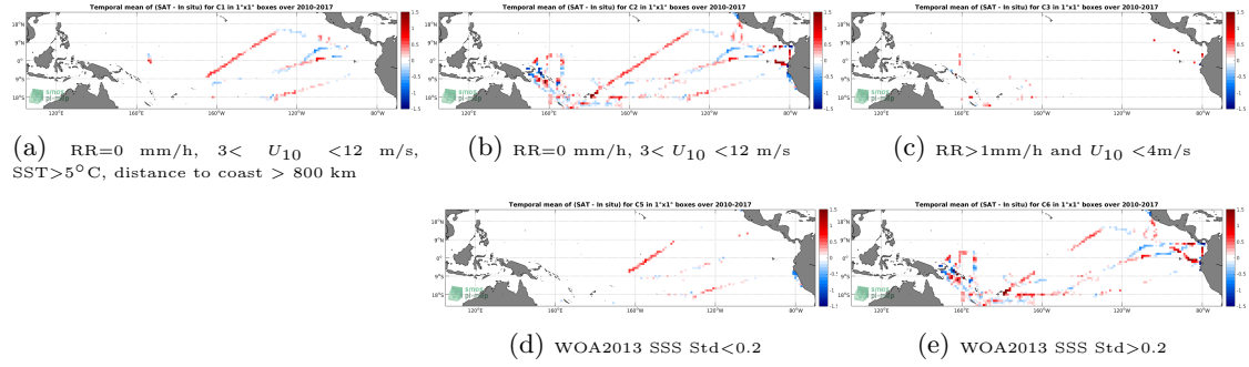
Figure 12: Temporal mean gridded over spatial boxes of size 1^{\circ}\times 1^{\circ} of \Delta SSS (SMOS L3 v2 - Monthly - 0.25 Deg (CATDS-CECOS-IFREMER) - TSG-GOSUD-Research-vessel) for 5 different subdatasets corresponding to:RR=0 mm/h, 3 < U_{10} < 12 m/s, SST >5^{\circ}\text{C} , distance to coast > 800 km (a), RR=0 mm/h, 3 < U_{10} < 12 m/s (b), RR >1 mm/h and U_{10} < 4 m/s (c), WOA2013 SSS Std <0.2 (d), WOA2013 SSS Std >0.2 (e).
