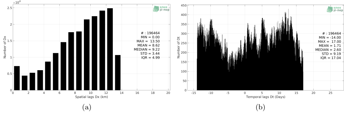
Figure 5: Histograms of the spatial (a) and temporal (b) lags between the time of the TSG-GOSUD-Research-vessel measurements and the date of the corresponding SMOS L3 v2 - Monthly - 0.25 Deg (CATDS-CECOS-IFREMER) SSS product.
