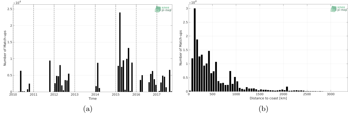
Figure 1: Number of match-ups between TSG-GOSUD-Research-vessel and SMOS L3 v2 - Monthly - 0.25 Deg (CATDS-CECOS-IFREMER) SSS as a function of time (a) and as function of the distance to coast (b) over the Tropical Pacific Ocean Pi-MEP region and for the full satellite product period.
