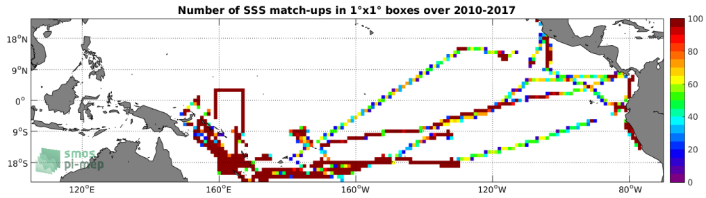
Figure 4: Number of SSS match-ups between TSG-GOSUD-Research-vessel SSS and the SMOS L3 v2 - Monthly - 0.25 Deg (CATDS-CECOS-IFREMER) SSS product for the Tropical Pacific Ocean Pi-MEP region over 1°x1° boxes and for the full satellite product period.
