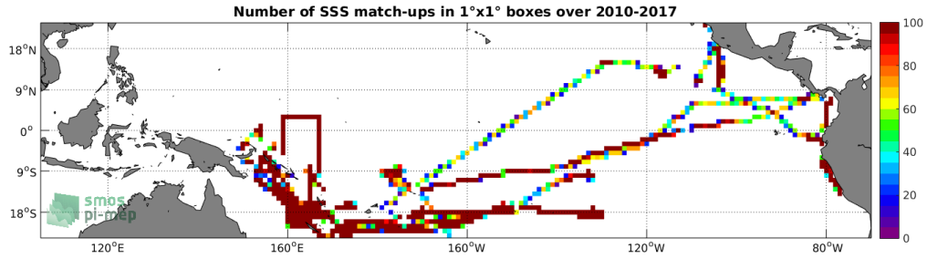
Figure 4: Number of SSS match-ups between TSG-GOSUD-Research-vessel SSS and the SMOS-L3-CATDS-IFREMER-CECOS-V2-MONTHLY-0.25DEG SSS product for the Tropical Pacific Ocean Pi-MEP region over 1°x1° boxes and for the full satellite product period.
