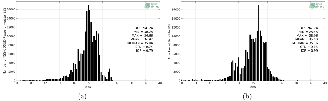
Figure 2: Histograms of SSS from TSG-GOSUD-Research-vessel (a) and SMOS-L3-CATDS-IFREMER-CECOS-V2-MONTHLY-0.25DEG (b) considering all match-up pairs per bins of 0.1 over the Tropical Pacific Ocean Pi-MEP region and for the full satellite product period.
