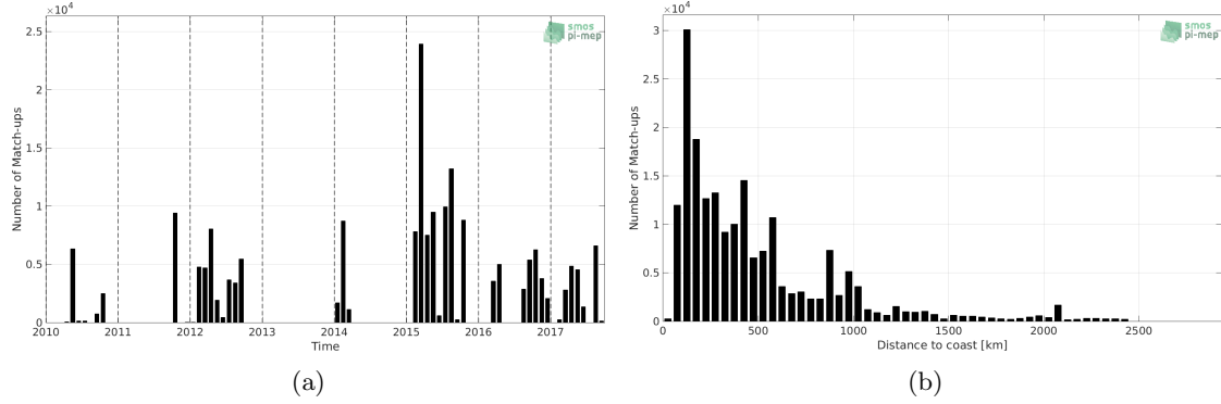
Figure 1: Number of match-ups between TSG-GOSUD-Research-vessel and SMOS-L3-CATDS-IFREMER-CECOS-V2-MONTHLY-0.25DEG SSS as a function of time (a) and as function of the distance to coast (b) over the Tropical Pacific Ocean Pi-MEP region and for the full satellite product period.
