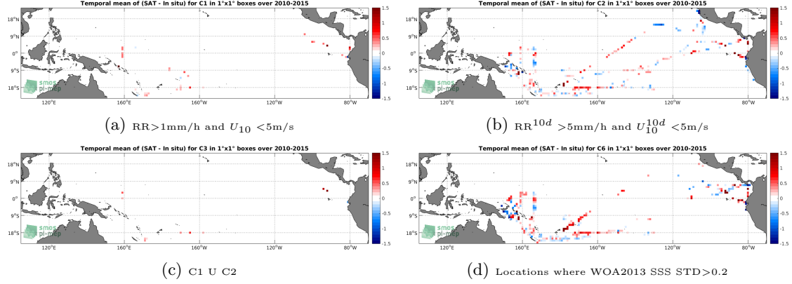
Figure 12: Temporal mean gridded over spatial boxes of size 1^\circ \times 1^\circ of \Delta SSS (SMOS-L3-CATDS-IFREMER-CECOS-V2-MONTHLY-0.25DEG - TSG-GOSUD-Research-vessel) for 4 different subdatasets corresponding to: RR > 1\text{mm/h} and U_{10} < 5\text{m/s} (a), RR^{10d} > 5\text{mm/h} and U_{10}^{10d} < 5\text{m/s} (b), C1 U C2 (c), Locations where WOA2013 SSS STD > 0.2 (d).
