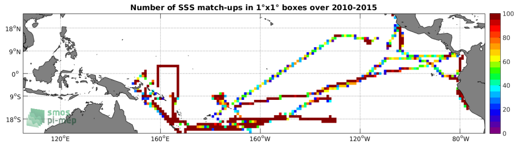
Figure 4: Number of SSS match-ups between TSG-GOSUD-Research-vessel SSS and the SMOS-L3-CATDS-IFREMER-CECOS-V2-MONTHLY-0.25DEG SSS product for the Tropical Pacific Ocean Pi-MEP region over 1^\circ \times 1^\circ boxes and for the full satellite product period.
