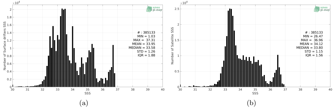
Figure 2: Histograms of SSS from Surface drifters (a) and SMOS SSS L3 v2 - Monthly - 0.25 Deg (CATDS-CECOS-IFREMER) (b) considering all match-up pairs per bins of 0.1 over the Tropical Pacific Ocean Pi-MEP region and for the full satellite product period.
