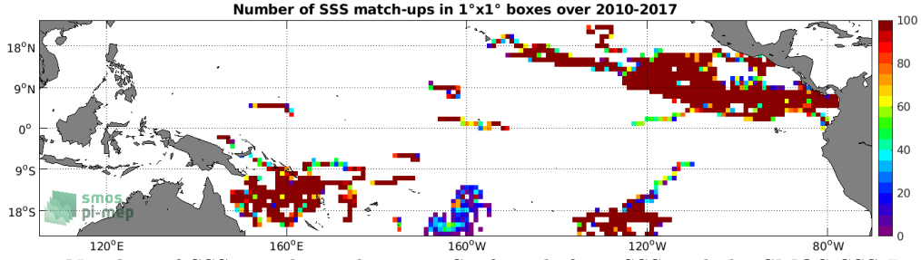
Figure 3: Number of SSS match-ups between Surface drifters SSS and the SMOS SSS L3 v2 - Monthly - 0.25 Deg (CATDS-CECOS-IFREMER) SSS product for the Tropical Pacific Ocean Pi-MEP region over 1^\circ \times 1^\circ boxes and for the full satellite product period.
