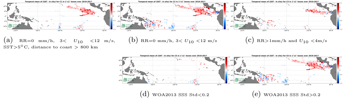
Figure 11: Temporal mean gridded over spatial boxes of size 1^{\circ}\times 1^{\circ} of \Delta\text{SSS} (SMOS SSS L3 v2 - Monthly - 0.25 Deg (CATDS-CECOS-IFREMER) - Surface drifters) for 5 different subdatasets corresponding to: RR=0 mm/h, 3 < U_{10} < 12 m/s, SST > 5^{\circ}\text{C} , distance to coast > 800 km (a), RR=0 mm/h, 3 < U_{10} < 12 m/s (b), RR > 1 mm/h and U_{10} < 4 m/s (c), WOA2013 SSS Std < 0.2 (d), WOA2013 SSS Std > 0.2 (e).
