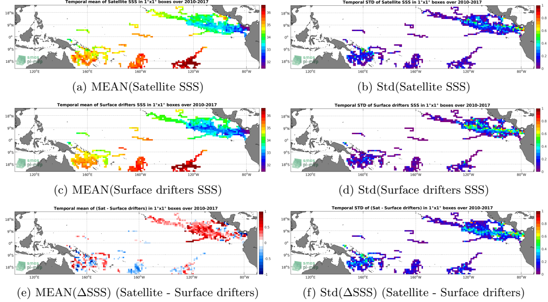
Figure 5: Temporal mean (left) and Std (right) of SSS from SMOS SSS L3 v2 - Monthly - 0.25 Deg (CATDS-CECOS-IFREMER) (top), Surface drifters (middle), and of \Delta SSS (Satellite - Surface drifters). Only match-up pairs are used to generate these maps.
