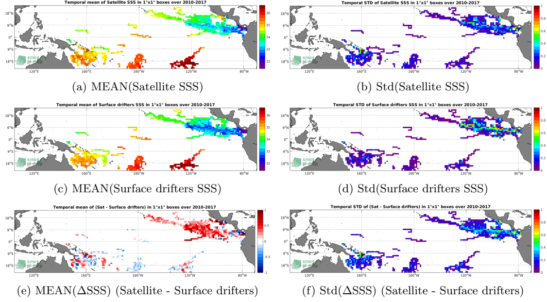
Figure 5: Temporal mean (left) and Std (right) of SSS from SMOS L3 v2 - Monthly - 0.25 Deg (CATDS-CECOS-IFREMER) (top), Surface drifters (middle), and of \Delta SSS (Satellite - Surface drifters). Only match-up pairs are used to generate these maps.
