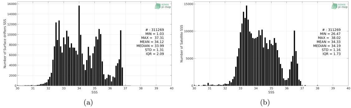
Figure 2: Histograms of SSS from Surface drifters (a) and SMOS L3 v2 - Monthly - 0.25 Deg (CATDS-CECOS-IFREMER) (b) considering all match-up pairs per bins of 0.1 over the Tropical Pacific Ocean Pi-MEP region and for the full satellite product period.
