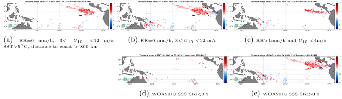
Figure 11: Temporal mean gridded over spatial boxes of size 1^{\circ}\times 1^{\circ} of \Delta\text{SSS} (SMOS L3 v2 - Monthly - 0.25 Deg (CATDS-CECOS-IFREMER) - Surface drifters) for 5 different subdatasets corresponding to: RR=0 mm/h, 3 < U_{10} < 12 m/s, SST > 5^{\circ}\text{C} , distance to coast > 800 km (a), RR=0 mm/h, 3 < U_{10} < 12 m/s (b), RR > 1 mm/h and U_{10} < 4 m/s (c), WOA2013 SSS Std < 0.2 (d), WOA2013 SSS Std > 0.2 (e).
