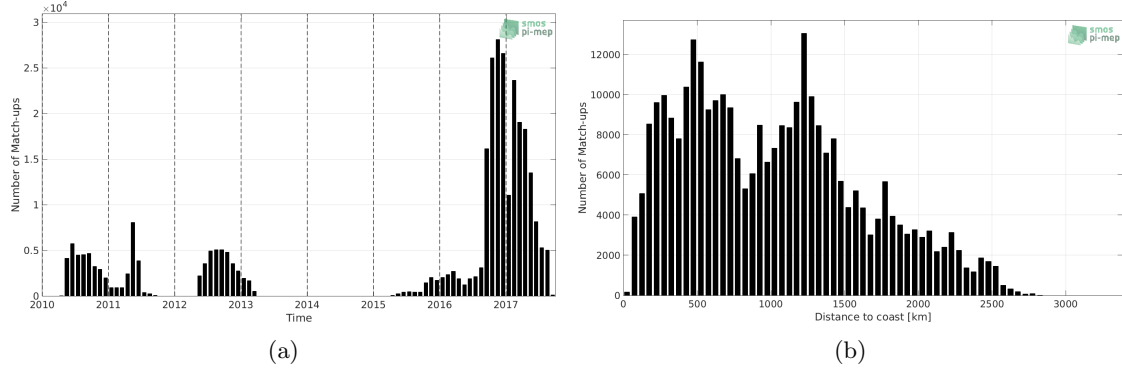
Figure 1: Number of match-ups between Surface drifters and SMOS L3 v2 - Monthly - 0.25 Deg (CATDS-CECOS-IFREMER) SSS as a function of time (a) and as function of the distance to coast (b) over the Tropical Pacific Ocean Pi-MEP region and for the full satellite product period.
