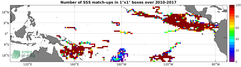
Figure 3: Number of SSS match-ups between Surface drifters SSS and the SMOS L3 v2 - Monthly - 0.25 Deg (CATDS-CECOS-IFREMER) SSS product for the Tropical Pacific Ocean Pi-MEP region over 1°x1° boxes and for the full satellite product period.
