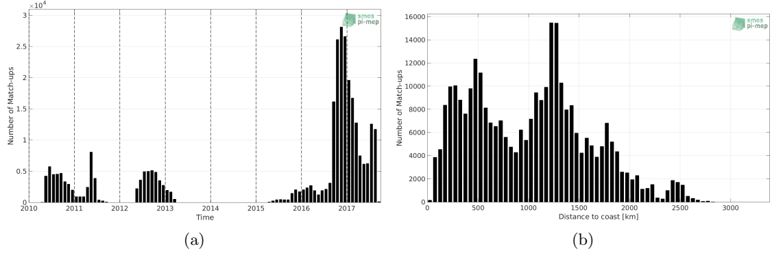
Figure 1: Number of match-ups between Surface drifters and SMOS-L3-CATDS-IFREMER-CECOS-V2-MONTHLY-0.25DEG SSS as a function of time (a) and as function of the distance to coast (b) over the Tropical Pacific Ocean Pi-MEP region and for the full satellite product period.
