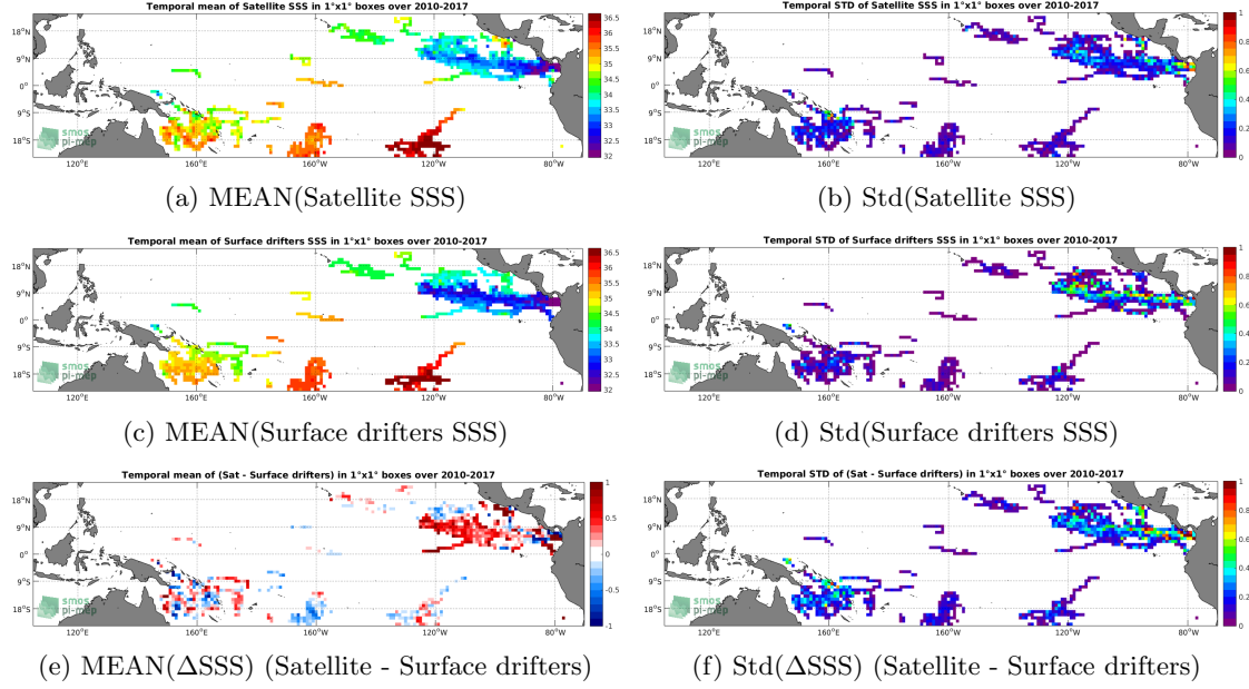
Figure 5: Temporal mean (left) and Std (right) of SSS from SMOS-L3-CATDS-IFREMER-CECOS-V2-MONTHLY-0.25DEG (top), Surface drifters (middle), and of \Delta SSS (Satellite - Surface drifters). Only match-up pairs are used to generate these maps.
