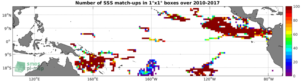
Figure 3: Number of SSS match-ups between Surface drifters SSS and the SMOS-L3-CATDS-IFREMER-CECOS-V2-MONTHLY-0.25DEG SSS product for the Tropical Pacific Ocean Pi-MEP region over 1^\circ \times 1^\circ boxes and for the full satellite product period.
