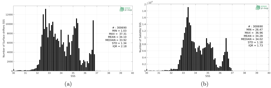
Figure 2: Histograms of SSS from Surface drifters (a) and SMOS-L3-CATDS-IFREMER-CECOS-V2-MONTHLY-0.25DEG (b) considering all match-up pairs per bins of 0.1 over the Tropical Pacific Ocean Pi-MEP region and for the full satellite product period.
