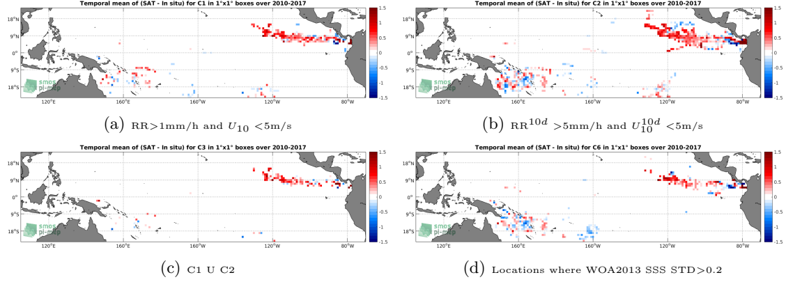
Figure 11: Temporal mean gridded over spatial boxes of size 1^\circ \times 1^\circ of \Delta SSS (SMOS-L3-CATDS-IFREMER-CECOS-V2-MONTHLY-0.25DEG - Surface drifters) for 4 different subdatasets corresponding to: RR > 1\text{mm/h} and U_{10} < 5\text{m/s} (a), RR^{10d} > 5\text{mm/h} and U_{10}^{10d} < 5\text{m/s} (b), C1 U C2 (c), Locations where WOA2013 SSS STD > 0.2 (d).
