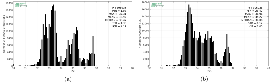
Figure 2: Histograms of SSS from Surface drifters (a) and SMOS-L3-CATDS-IFREMER-CECOS-V2-MONTHLY-0.25DEG (b) considering all match-up pairs per bins of 0.1 over the Tropical Pacific Ocean Pi-MEP region and for the full satellite product period.
