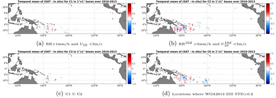
Figure 11: Temporal mean gridded over spatial boxes of size 1^\circ \times 1^\circ of \Delta SSS (SMOS-L3-CATDS-IFREMER-CECOS-V2-MONTHLY-0.25DEG - Surface drifters) for 4 different subdatasets corresponding to: RR > 1\text{mm/h} and U_{10} < 5\text{m/s} (a), RR^{10d} > 5\text{mm/h} and U_{10}^{10d} < 5\text{m/s} (b), C1 U C2 (c), Locations where WOA2013 SSS STD > 0.2 (d).
