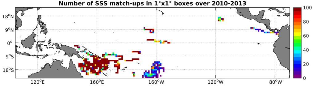
Figure 3: Number of SSS match-ups between Surface drifters SSS and the SMOS-L3-CATDS-IFREMER-CECOS-V2-MONTHLY-0.25DEG SSS product for the Tropical Pacific Ocean Pi-MEP region over 1^\circ \times 1^\circ boxes and for the full satellite product period.
