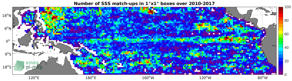
Figure 4: Number of SSS match-ups between Argo SSS and the SMOS SSS L3 v2 - Monthly - 0.25 Deg (CATDS-CECOS-IFREMER) SSS product for the Tropical Pacific Ocean Pi-MEP region over 1^\circ \times 1^\circ boxes and for the full satellite product period.
