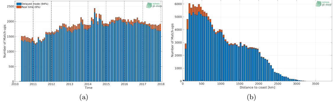
Figure 1: Number of match-ups between Argo and SMOS SSS L3 v2 - Monthly - 0.25 Deg (CATDS-CECOS-IFREMER) SSS as a function of time (a) and as function of the distance to coast (b) over the Tropical Pacific Ocean Pi-MEP region and for the full satellite product period.
