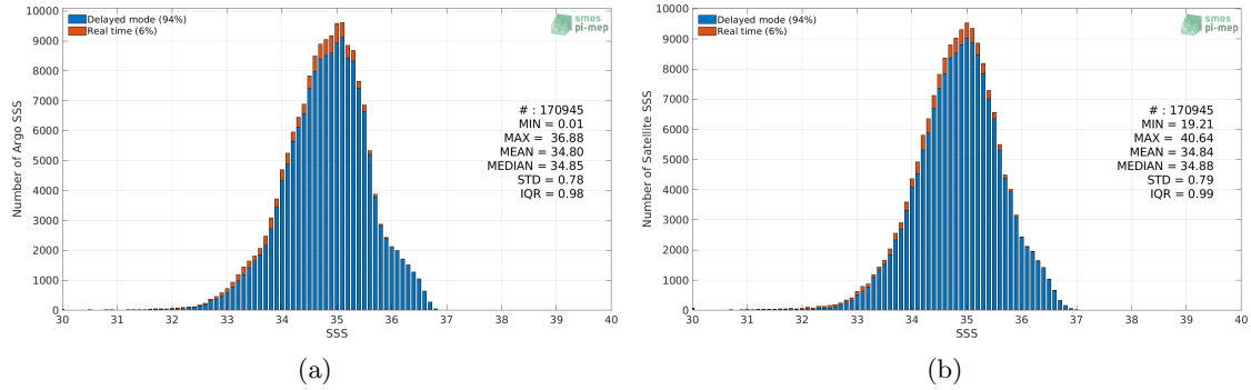
Figure 2: Histograms of SSS from Argo (a) and SMOS SSS L3 v2 - Monthly - 0.25 Deg (CATDS-CECOS-IFREMER) (b) considering all match-up pairs per bins of 0.1 over the Tropical Pacific Ocean Pi-MEP region and for the full satellite product period.
