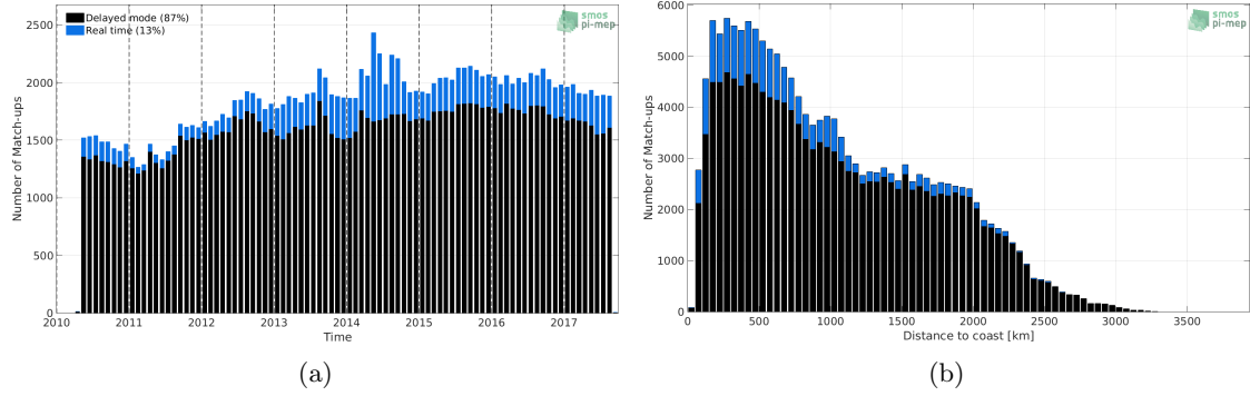
Figure 1: Number of match-ups between Argo and SMOS L3 v2 - Monthly - 0.25 Deg (CATDS-CECOS-IFREMER) SSS as a function of time (a) and as function of the distance to coast (b) over the Tropical Pacific Ocean Pi-MEP region and for the full satellite product period.
