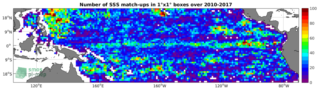
Figure 4: Number of SSS match-ups between Argo SSS and the SMOS L3 v2 - Monthly - 0.25 Deg (CATDS-CECOS-IFREMER) SSS product for the Tropical Pacific Ocean Pi-MEP region over 1°x1° boxes and for the full satellite product period.
