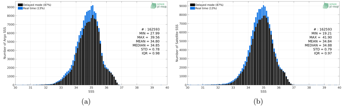
Figure 2: Histograms of SSS from Argo (a) and SMOS L3 v2 - Monthly - 0.25 Deg (CATDS-CECOS-IFREMER) (b) considering all match-up pairs per bins of 0.1 over the Tropical Pacific Ocean Pi-MEP region and for the full satellite product period.
