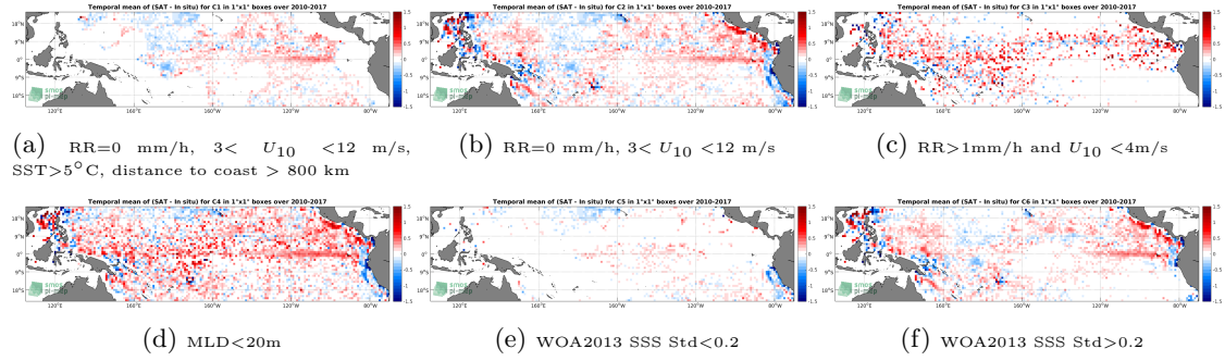
Figure 12: Temporal mean gridded over spatial boxes of size 1^\circ \times 1^\circ of \Delta SSS (SMOS L3 v2 - Monthly - 0.25^\circ Deg (CATDS-CECOS-IFREMER) - Argo) for 6 different subdatasets corresponding to: RR=0 mm/h, 3 < U_{10} < 12 m/s, SST > 5^\circ C , distance to coast > 800 km (a), RR=0 mm/h, 3 < U_{10} < 12 m/s (b), RR > 1 mm/h and U_{10} < 4 m/s (c), MLD < 20 m (d), WOA2013 SSS Std < 0.2 (e), WOA2013 SSS Std > 0.2 (f).
