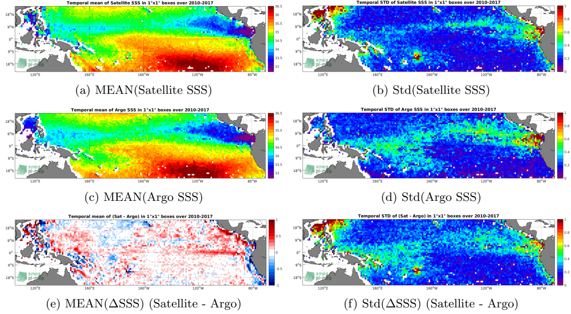
Figure 6: Temporal mean (left) and Std (right) of SSS from SMOS L3 v2 - Monthly - 0.25 Deg (CATDS-CECOS-IFREMER) (top), Argo (middle), and of \Delta SSS (Satellite - Argo). Only match-up pairs are used to generate these maps.
