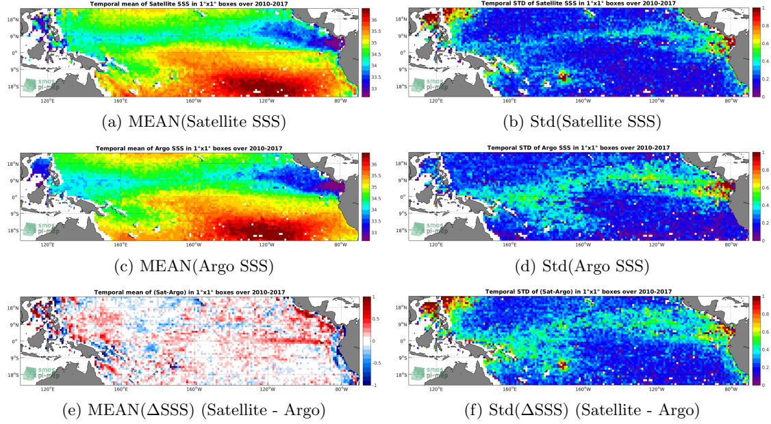
Figure 6: Temporal mean (left) and Std (right) of SSS from SMOS-L3-CATDS-IFREMER-CECOS-V2-MONTHLY-0.25DEG (top), Argo (middle), and of \Delta SSS (Satellite - Argo). Only match-up pairs are used to generate these maps.
