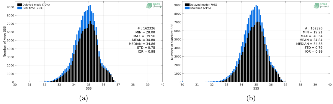
Figure 2: Histograms of SSS from Argo (a) and SMOS-L3-CATDS-IFREMER-CECOS-V2-MONTHLY-0.25DEG (b) considering all match-up pairs per bins of 0.1 over the Tropical Pacific Ocean Pi-MEP region and for the full satellite product period.
