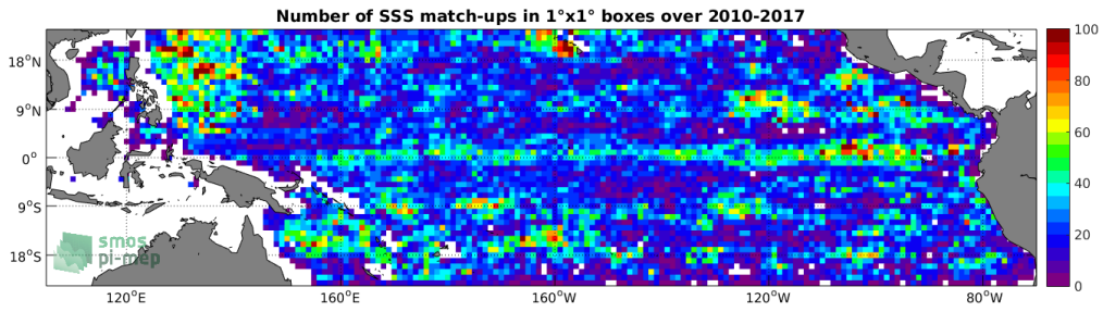
Figure 4: Number of SSS match-ups between Argo SSS and the SMOS-L3-CATDS-IFREMER-CECOS-V2-MONTHLY-0.25DEG SSS product for the Tropical Pacific Ocean Pi-MEP region over 1^\circ \times 1^\circ boxes and for the full satellite product period.
