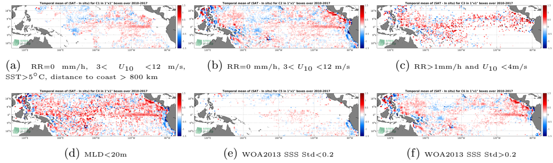
Figure 12: Temporal mean gridded over spatial boxes of size 1^\circ \times 1^\circ of \Delta SSS (SMOS-L3-CATDS-IFREMER-CECOS-V2-MONTHLY-0.25DEG - Argo) for 6 different subdatasets corresponding to: RR=0 mm/h, 3 < U_{10} < 12 m/s, SST > 5^\circ C , distance to coast > 800 km (a), RR=0 mm/h, 3 < U_{10} < 12 m/s (b), RR > 1 mm/h and U_{10} < 4 m/s (c), MLD < 20 m (d), WOA2013 SSS Std < 0.2 (e), WOA2013 SSS Std > 0.2 (f).
