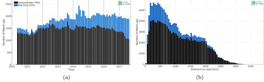
Figure 1: Number of match-ups between Argo and SMOS-L3-CATDS-IFREMER-CECOS-V2-MONTHLY-0.25DEG SSS as a function of time (a) and as function of the distance to coast (b) over the Tropical Pacific Ocean Pi-MEP region and for the full satellite product period.
