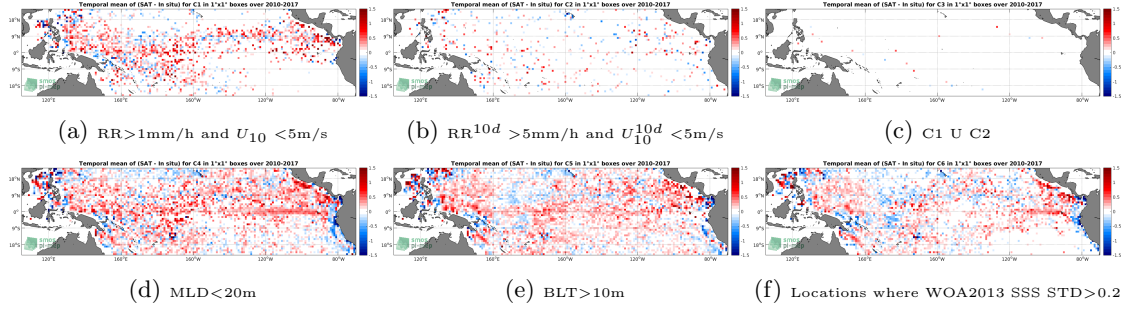
Figure 12: Temporal mean gridded over spatial boxes of size 1^\circ \times 1^\circ of \Delta\text{SSS} (SMOS-L3-CATDS-IFREMER-CECOS-V2-MONTHLY-0.25DEG - Argo) for 6 different subdatasets corresponding to: \text{RR}>1\text{mm/h} and U_{10}<5\text{m/s} (a), \text{RR}^{10d}>5\text{mm/h} and U_{10d}<5\text{m/s} (b), C1 U C2 (c), \text{MLD}<20\text{m} (d), \text{BLT}>10\text{m} (e), Locations where WOA2013 SSS STD >0.2 (f).
