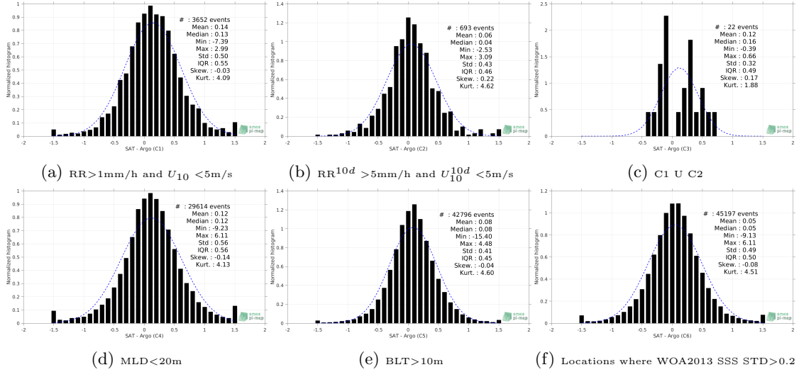
Figure 13: Normalized histogram of \Delta\text{SSS} (SMOS-L3-CATDS-IFREMER-CECOS-V2-MONTHLY-0.25DEG - Argo) for 6 different subdatasets corresponding to: \text{RR}>1\text{mm/h} and U_{10}<5\text{m/s} (a), \text{RR}^{10d}>5\text{mm/h} and U_{10d}<5\text{m/s} (b), C1 U C2 (c), \text{MLD}<20\text{m} (d), \text{BLT}>10\text{m} (e), Locations where WOA2013 SSS STD >0.2 (f).
