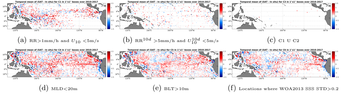
Figure 12: Temporal mean gridded over spatial boxes of size 1^\circ \times 1^\circ of \Delta SSS (SMOS-L3-CATDS-IFREMER-CECOS-V2-MONTHLY-0.25DEG - Argo) for 6 different subdatasets corresponding to: RR > 1\text{mm/h} and U_{10} < 5\text{m/s} (a), RR^{10d} > 5\text{mm/h} and U_{10}^{10d} < 5\text{m/s} (b), C1 U C2 (c), MLD < 20\text{m} (d), BLT > 10\text{m} (e), Locations where WOA2013 SSS STD > 0.2 (f).
