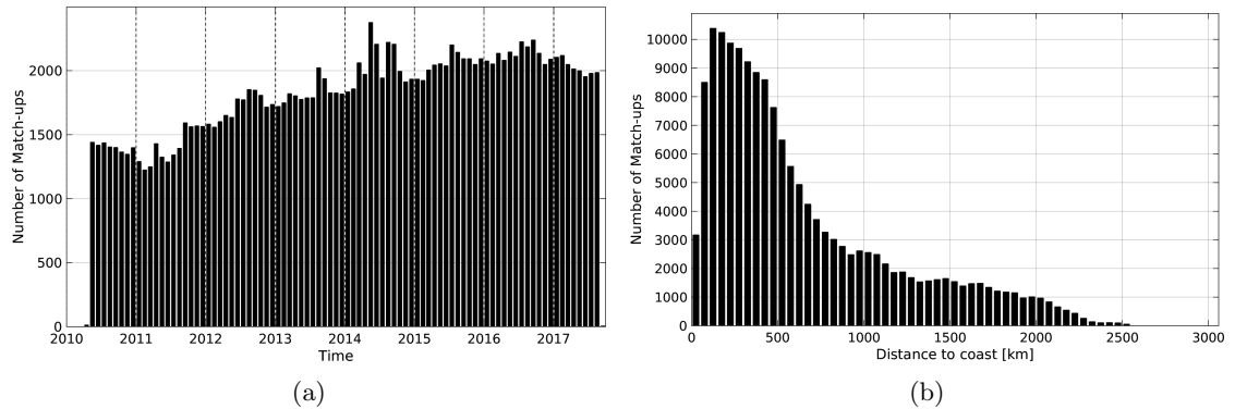
Figure 1: Number of match-ups between Argo and SMOS-L3-CATDS-IFREMER-CECOS-V2-MONTHLY-0.25DEG SSS as a function of time (a) and as function of the distance to coast (b) over the Tropical Pacific Ocean Pi-MEP region and for the full satellite product period.
