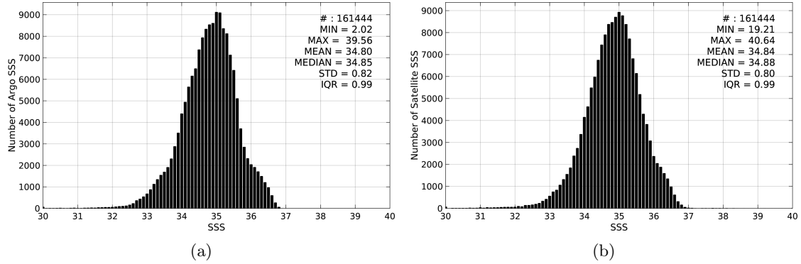
Figure 2: Histograms of SSS from Argo (a) and SMOS-L3-CATDS-IFREMER-CECOS-V2-MONTHLY-0.25DEG (b) considering all match-up pairs per bins of 0.1 over the Tropical Pacific Ocean Pi-MEP region and for the full satellite product period.
