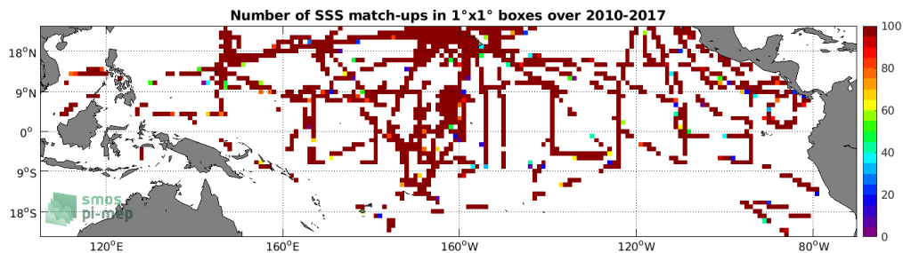
Figure 4: Number of SSS match-ups between TSG (SAMOS) SSS and the SMOS SSS L3 v2 - Daily - 0.5 Deg (CATDS-CECOS-IFREMER) SSS product for the Tropical Pacific Ocean Pi-MEP region over 1^\circ \times 1^\circ boxes and for the full satellite product period.
