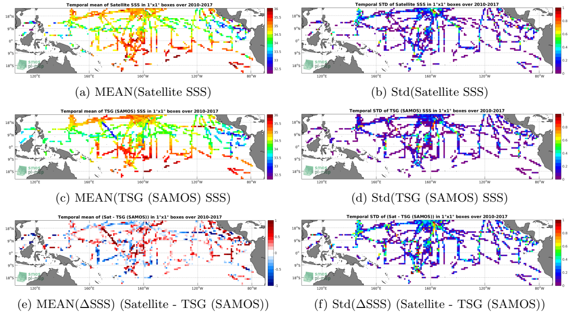
Figure 6: Temporal mean (left) and Std (right) of SSS from SMOS SSS L3 v2 - Daily - 0.5 Deg (CATDS-CECOS-IFREMER) (top), TSG (SAMOS) (middle), and of \Delta SSS (Satellite - TSG (SAMOS)). Only match-up pairs are used to generate these maps.
