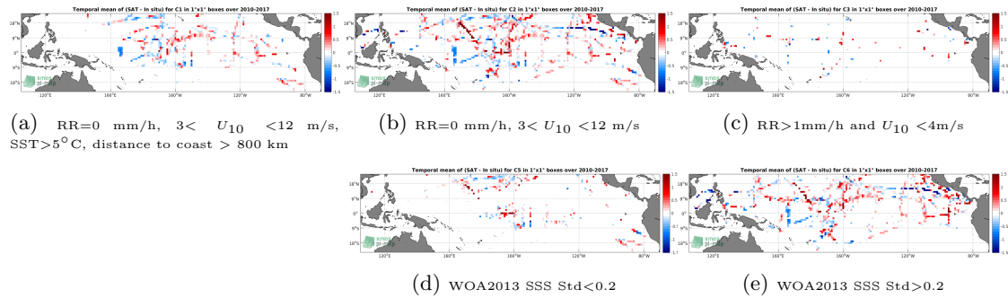
Figure 12: Temporal mean gridded over spatial boxes of size 1^{\circ}\times 1^{\circ} of \Delta\text{SSS} (SMOS SSS L3 v2 - Daily - 0.5 Deg (CATDS-CECOS-IFREMER) - TSG (SAMOS)) for 5 different subdatasets corresponding to:RR=0 mm/h, 3 < U_{10} < 12 m/s, SST > 5^{\circ}\text{C} , distance to coast > 800 km (a), RR=0 mm/h, 3 < U_{10} < 12 m/s (b), RR > 1 mm/h and U_{10} < 4 m/s (c), WOA2013 SSS Std < 0.2 (d), WOA2013 SSS Std > 0.2 (e).
