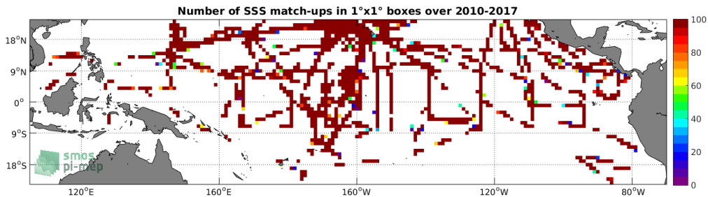
Figure 4: Number of SSS match-ups between TSG (SAMOS) SSS and the SMOS SSS L3 v2 - Daily - 0.5 Deg (CATDS-CECOS-IFREMER) SSS product for the Tropical Pacific Ocean Pi-MEP region over 1^\circ \times 1^\circ boxes and for the full satellite product period.
