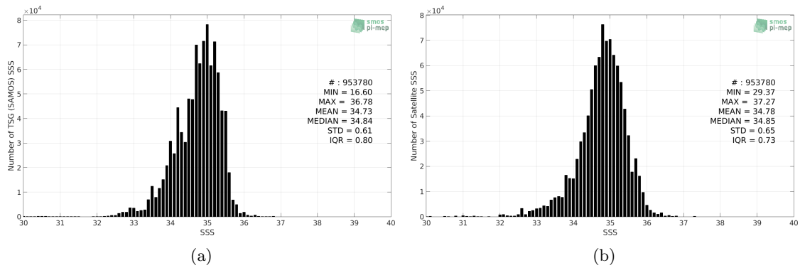
Figure 2: Histograms of SSS from TSG (SAMOS) (a) and SMOS SSS L3 v2 - Daily - 0.5 Deg (CATDS-CECOS-IFREMER) (b) considering all match-up pairs per bins of 0.1 over the Tropical Pacific Ocean Pi-MEP region and for the full satellite product period.
