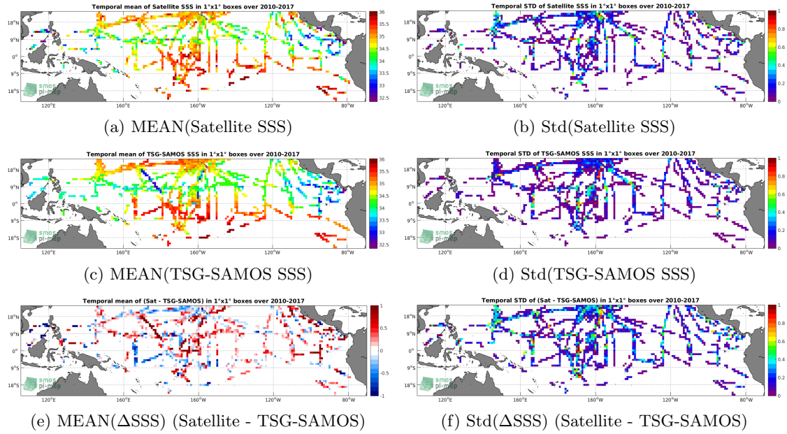
Figure 6: Temporal mean (left) and Std (right) of SSS from SMOS L3 v2 - Daily - 0.5 Deg (CATDS-CECOS-IFREMER) (top), TSG-SAMOS (middle), and of \Delta SSS (Satellite - TSG-SAMOS). Only match-up pairs are used to generate these maps.
