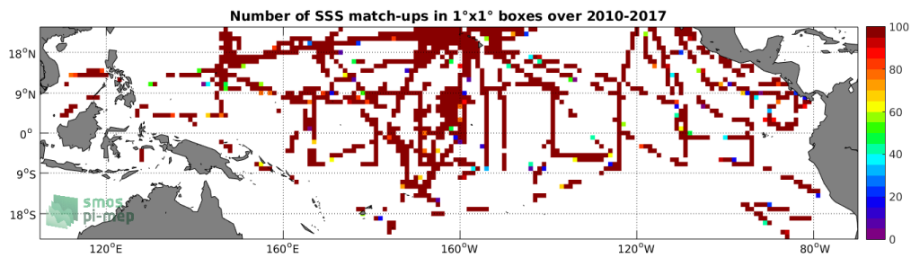
Figure 4: Number of SSS match-ups between TSG-SAMOS SSS and the SMOS L3 v2 - Daily - 0.5 Deg (CATDS-CECOS-IFREMER) SSS product for the Tropical Pacific Ocean Pi-MEP region over 1^\circ \times 1^\circ boxes and for the full satellite product period.
