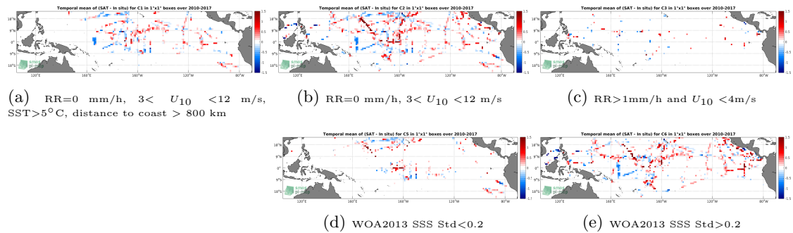
Figure 12: Temporal mean gridded over spatial boxes of size 1^\circ \times 1^\circ of \Delta SSS (SMOS L3 v2 - Daily - 0.5 Deg (CATDS-CECOS-IFREMER) - TSG-SAMOS) for 5 different subdatasets corresponding to: RR=0 mm/h, 3 < U_{10} < 12 m/s, SST > 5^\circ\text{C} , distance to coast > 800 km (a), RR=0 mm/h, 3 < U_{10} < 12 m/s (b), RR > 1 mm/h and U_{10} < 4 m/s (c), WOA2013 SSS Std < 0.2 (d), WOA2013 SSS Std > 0.2 (e).
