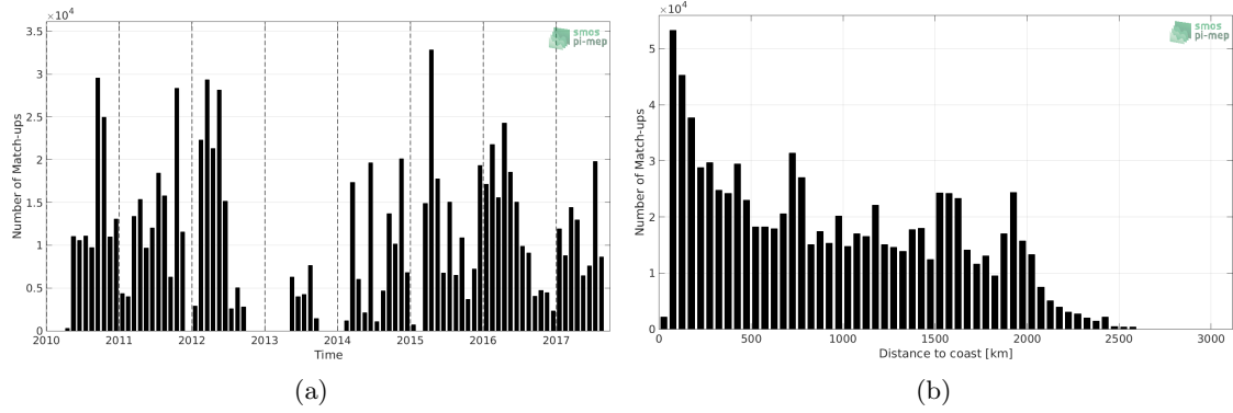
Figure 1: Number of match-ups between TSG-SAMOS and SMOS L3 v2 - Daily - 0.5 Deg (CATDS-CECOS-IFREMER) SSS as a function of time (a) and as function of the distance to coast (b) over the Tropical Pacific Ocean Pi-MEP region and for the full satellite product period.
