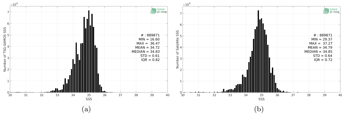
Figure 2: Histograms of SSS from TSG-SAMOS (a) and SMOS L3 v2 - Daily - 0.5 Deg (CATDS-CECOS-IFREMER) (b) considering all match-up pairs per bins of 0.1 over the Tropical Pacific Ocean Pi-MEP region and for the full satellite product period.
