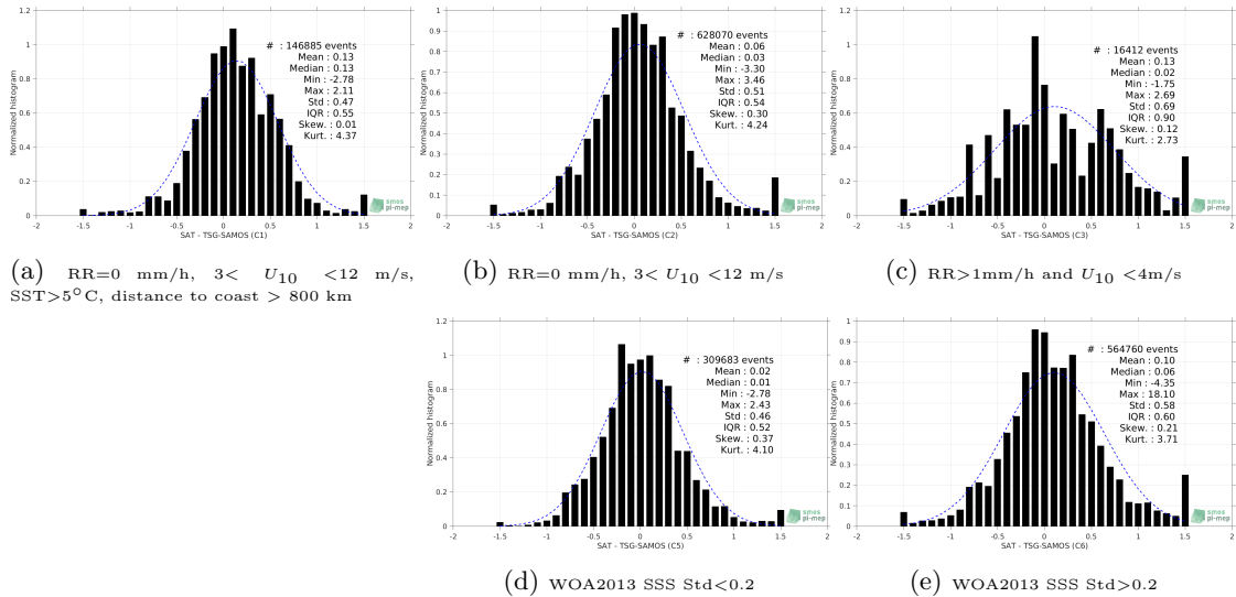
Figure 13: Normalized histogram of \Delta SSS (SMOS-L3-CATDS-CECOS-IFREMER-V2-1DAY-0.5DEG - TSG-SAMOS) for 5 different subdatasets corresponding to: RR=0 mm/h, 3 < U_{10} < 12 m/s, SST >5^\circ C, distance to coast > 800 km (a), RR=0 mm/h, 3 < U_{10} < 12 m/s (b), RR >1 mm/h and U_{10} < 4 m/s (c), WOA2013 SSS Std <0.2 (d), WOA2013 SSS Std >0.2 (e).
