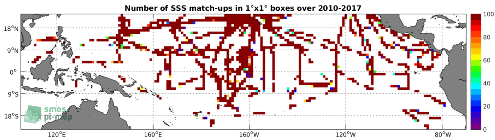
Figure 4: Number of SSS match-ups between TSG-SAMOS SSS and the SMOS-L3-CATDS-CECOS-IFREMER-V2-1DAY-0.5DEG SSS product for the Tropical Pacific Ocean Pi-MEP region over 1^\circ \times 1^\circ boxes and for the full satellite product period.
