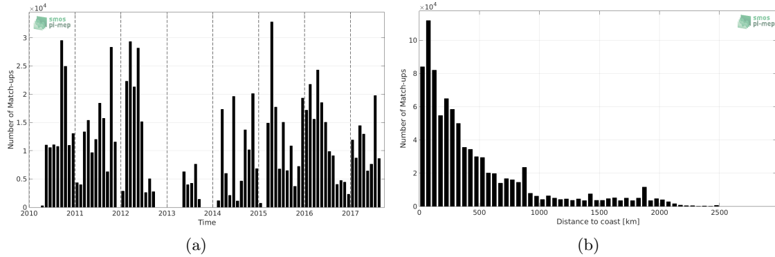
Figure 1: Number of match-ups between TSG-SAMOS and SMOS-L3-CATDS-CECOS-IFREMER-V2-1DAY-0.5DEG SSS as a function of time (a) and as function of the distance to coast (b) over the Tropical Pacific Ocean Pi-MEP region and for the full satellite product period.
