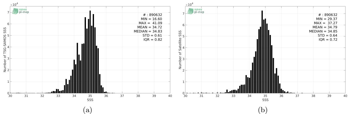
Figure 2: Histograms of SSS from TSG-SAMOS (a) and SMOS-L3-CATDS-CECOS-IFREMER-V2-1DAY-0.5DEG (b) considering all match-up pairs per bins of 0.1 over the Tropical Pacific Ocean Pi-MEP region and for the full satellite product period.
