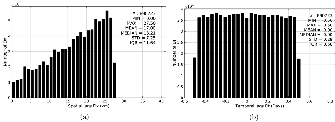
Figure 5: Histograms of the spatial (a) and temporal (b) lags between the time of the TSG-SAMOS measurements and the date of the corresponding SMOS-L3-CATDS-CECOS-IFREMER-V2-1DAY-0.5DEG SSS product.
