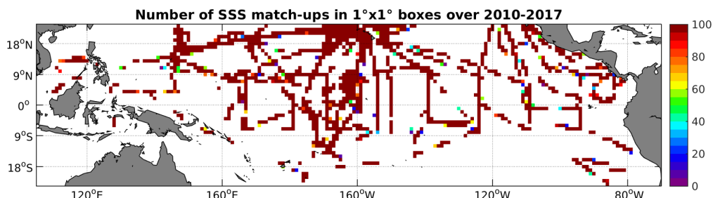
Figure 4: Number of SSS match-ups between TSG-SAMOS SSS and the SMOS-L3-CATDS-CECOS-IFREMER-V2-1DAY-0.5DEG SSS product for the Tropical Pacific Ocean Pi-MEP region over 1^\circ \times 1^\circ boxes and for the full satellite product period.
