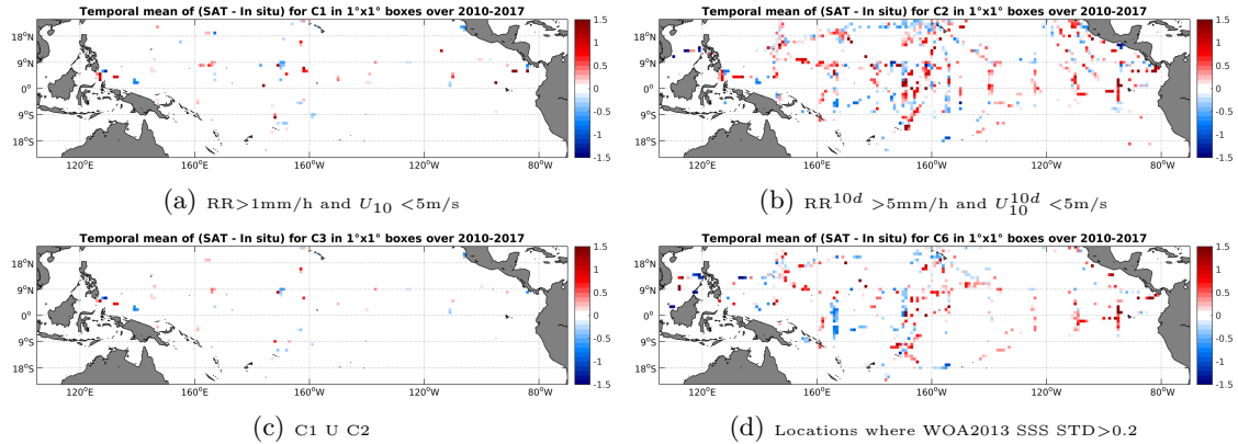
Figure 12: Temporal mean gridded over spatial boxes of size 1^\circ \times 1^\circ of \Delta SSS (SMOS-L3-CATDS-CECOS-IFREMER-V2-1DAY-0.5DEG - TSG-SAMOS) for 4 different subdatasets corresponding to: RR > 1\text{mm/h} and U_{10} < 5\text{m/s} (a), RR^{10d} > 5\text{mm/h} and U_{10}^{10d} < 5\text{m/s} (b), C1 U C2 (c), Locations where WOA2013 SSS STD > 0.2 (d).
