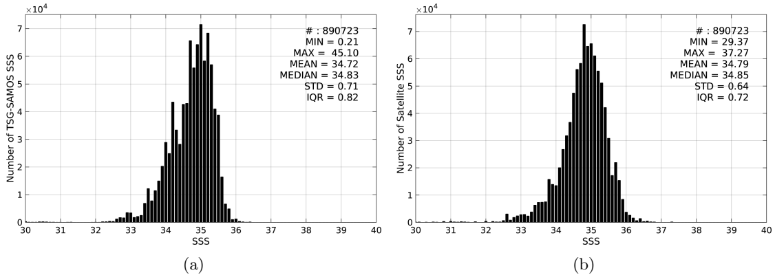
Figure 2: Histograms of SSS from TSG-SAMOS (a) and SMOS-L3-CATDS-CECOS-IFREMER-V2-1DAY-0.5DEG (b) considering all match-up pairs per bins of 0.1 over the Tropical Pacific Ocean Pi-MEP region and for the full satellite product period.
