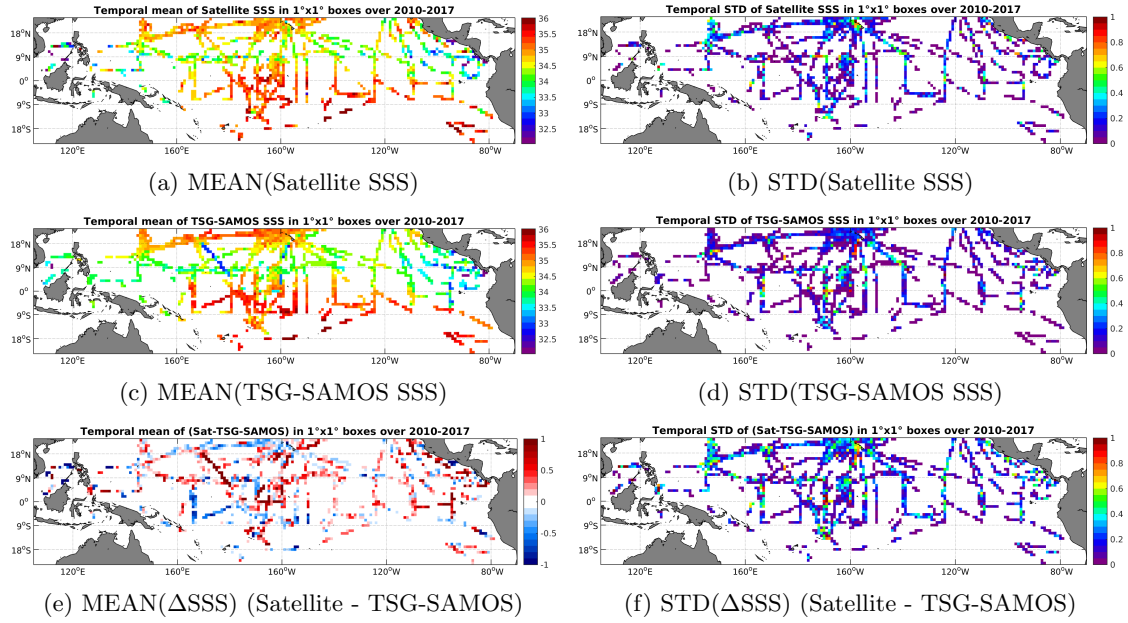
Figure 6: Temporal mean (left) and STD (right) of SSS from SMOS-L3-CATDS-CECOS-IFREMER-V2-1DAY-0.5DEG (top), TSG-SAMOS (middle), and of \Delta SSS (Satellite - TSG-SAMOS). Only match-up pairs are used to generate these maps.
