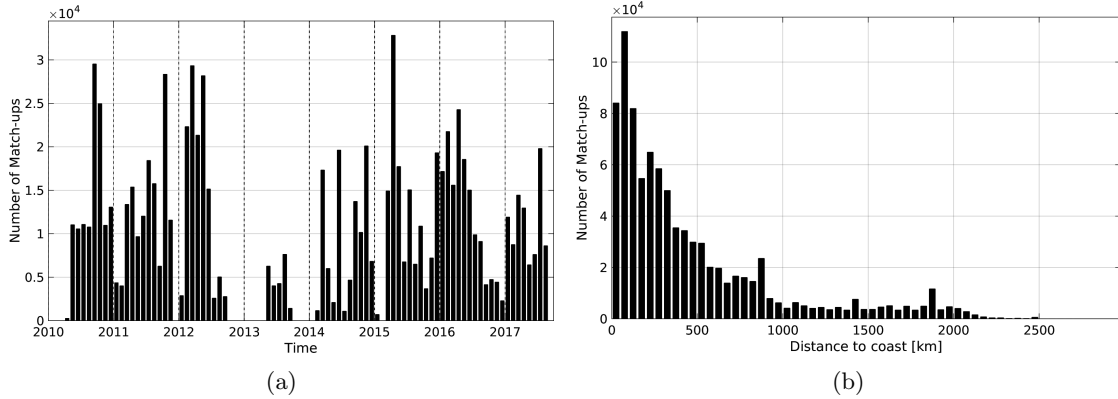
Figure 1: Number of match-ups between TSG-SAMOS and SMOS-L3-CATDS-CECOS-IFREMER-V2-1DAY-0.5DEG SSS as a function of time (a) and as function of the distance to coast (b) over the Tropical Pacific Ocean Pi-MEP region and for the full satellite product period.
