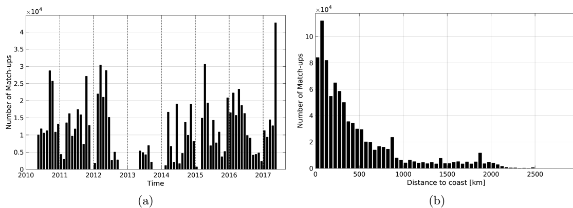
Figure 1: Number of match-ups between TSG-SAMOS and SMOS-L3-CATDS-CECOS-IFREMER-V2-1DAY-0.5deg SSS as a function of time (a) and as function of the distance to coast (b) over the Tropical Pacific Ocean Pi-MEP region and for the full satellite product period.
