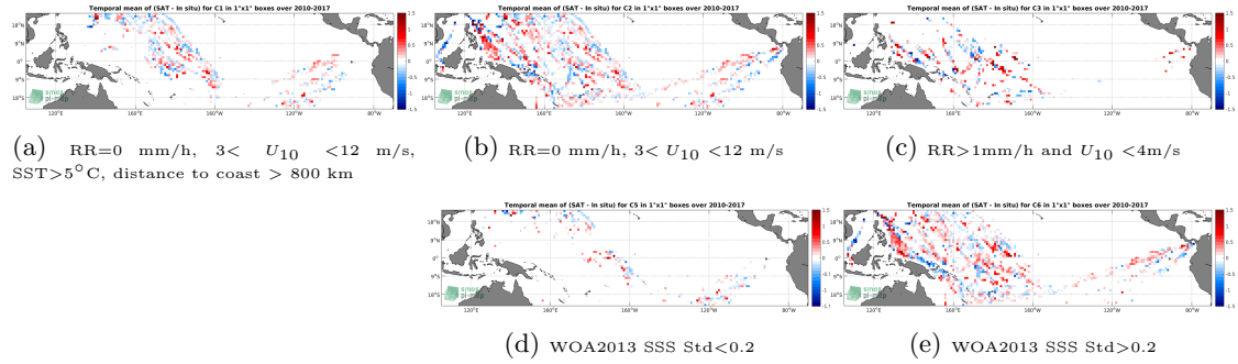
Figure 12: Temporal mean gridded over spatial boxes of size 1^{\circ}\times 1^{\circ} of \Delta\text{SSS} (SMOS SSS L3 v2 - Daily - 0.5 Deg (CATDS-CECOS-IFREMER) - TSG (LEGOS-DM)) for 5 different subdatasets corresponding to: RR=0 mm/h, 3 < U_{10} < 12 m/s, SST > 5^{\circ}\text{C} , distance to coast > 800 km (a), RR=0 mm/h, 3 < U_{10} < 12 m/s (b), RR > 1 mm/h and U_{10} < 4 m/s (c), WOA2013 SSS Std < 0.2 (d), WOA2013 SSS Std > 0.2 (e).
