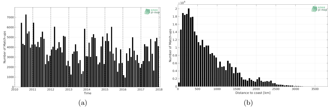
Figure 1: Number of match-ups between TSG (LEGOS-DM) and SMOS SSS L3 v2 - Daily - 0.5 Deg (CATDS-CECOS-IFREMER) SSS as a function of time (a) and as function of the distance to coast (b) over the Tropical Pacific Ocean Pi-MEP region and for the full satellite product period.
