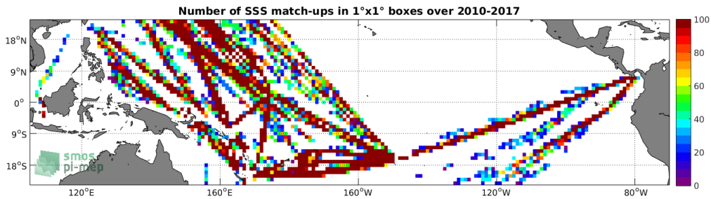
Figure 4: Number of SSS match-ups between TSG (LEGOS-DM) SSS and the SMOS SSS L3 v2 - Daily - 0.5 Deg (CATDS-CECOS-IFREMER) SSS product for the Tropical Pacific Ocean Pi-MEP region over 1^\circ \times 1^\circ boxes and for the full satellite product period.
