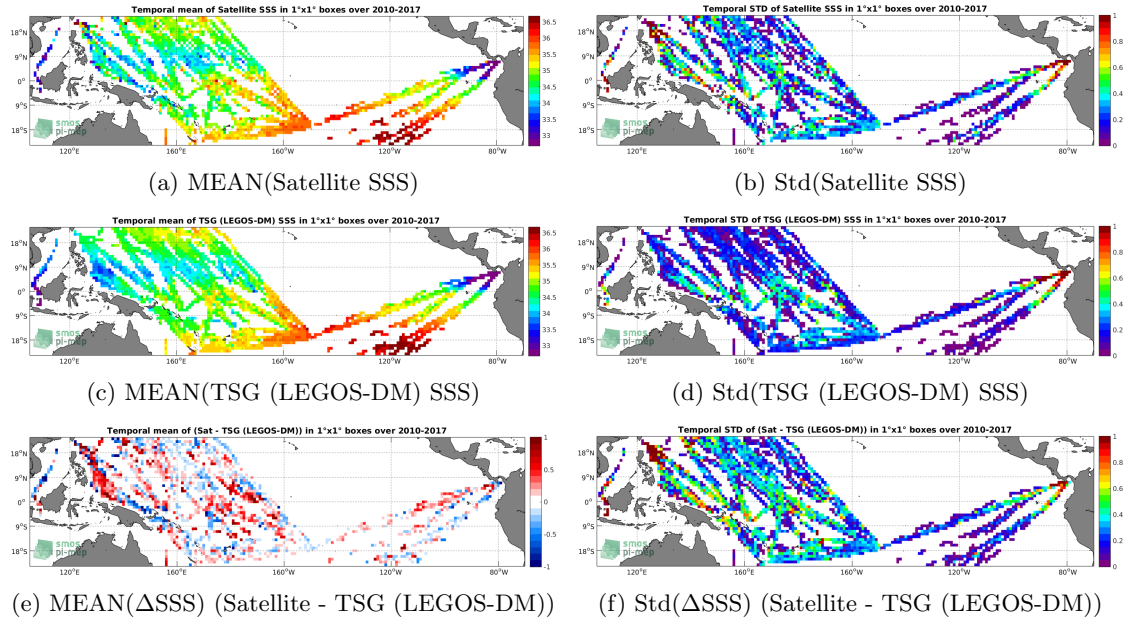
Figure 6: Temporal mean (left) and Std (right) of SSS from SMOS SSS L3 v2 - Daily - 0.5 Deg (CATDS-CECOS-IFREMER) (top), TSG (LEGOS-DM) (middle), and of \Delta SSS (Satellite - TSG (LEGOS-DM)). Only match-up pairs are used to generate these maps.
