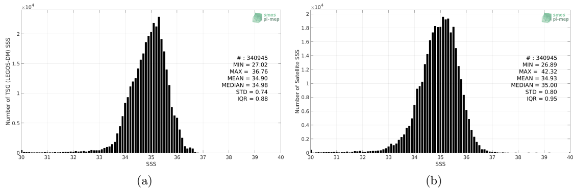
Figure 2: Histograms of SSS from TSG (LEGOS-DM) (a) and SMOS SSS L3 v2 - Daily - 0.5 Deg (CATDS-CECOS-IFREMER) (b) considering all match-up pairs per bins of 0.1 over the Tropical Pacific Ocean Pi-MEP region and for the full satellite product period.
