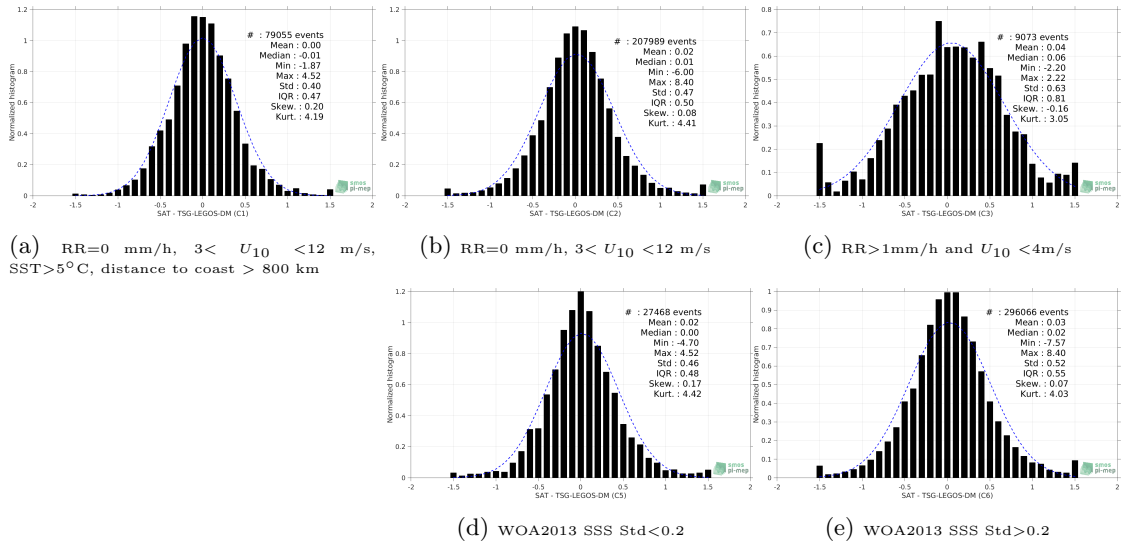
Figure 13: Normalized histogram of \Delta SSS (SMOS-L3-CATDS-CECOS-IFREMER-V2-1DAY-0.5DEG - TSG-LEGOS-DM) for 5 different subdatasets corresponding to: RR=0 mm/h, 3 < U_{10} < 12 m/s, SST >5^\circ C, distance to coast > 800 km (a), RR=0 mm/h, 3 < U_{10} < 12 m/s (b), RR >1 mm/h and U_{10} < 4 m/s (c), WOA2013 SSS Std <0.2 (d), WOA2013 SSS Std >0.2 (e).
