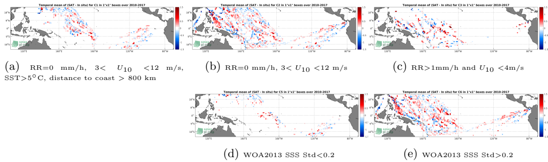
Figure 12: Temporal mean gridded over spatial boxes of size 1^\circ \times 1^\circ of \Delta SSS (SMOS-L3-CATDS-CECOS-IFREMER-V2-1DAY-0.5DEG - TSG-LEGOS-DM) for 5 different subdatasets corresponding to: RR=0 mm/h, 3 < U_{10} < 12 m/s, SST >5^\circ C, distance to coast > 800 km (a), RR=0 mm/h, 3 < U_{10} < 12 m/s (b), RR >1 mm/h and U_{10} < 4 m/s (c), WOA2013 SSS Std <0.2 (d), WOA2013 SSS Std >0.2 (e).
