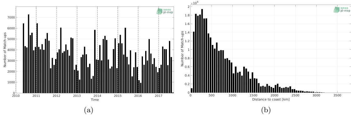
Figure 1: Number of match-ups between TSG-LEGOS-DM and SMOS-L3-CATDS-CECOS-IFREMER-V2-1DAY-0.5DEG SSS as a function of time (a) and as function of the distance to coast (b) over the Tropical Pacific Ocean Pi-MEP region and for the full satellite product period.
