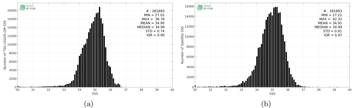
Figure 2: Histograms of SSS from TSG-LEGOS-DM (a) and SMOS-L3-CATDS-CECOS-IFREMER-V2-1DAY-0.5DEG (b) considering all match-up pairs per bins of 0.1 over the Tropical Pacific Ocean Pi-MEP region and for the full satellite product period.
