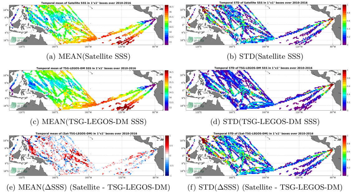
Figure 6: Temporal mean (left) and STD (right) of SSS from SMOS-L3-CATDS-CECOS-IFREMER-V2-1DAY-0.5DEG (top), TSG-LEGOS-DM (middle), and of \Delta SSS (Satellite - TSG-LEGOS-DM). Only match-up pairs are used to generate these maps.
