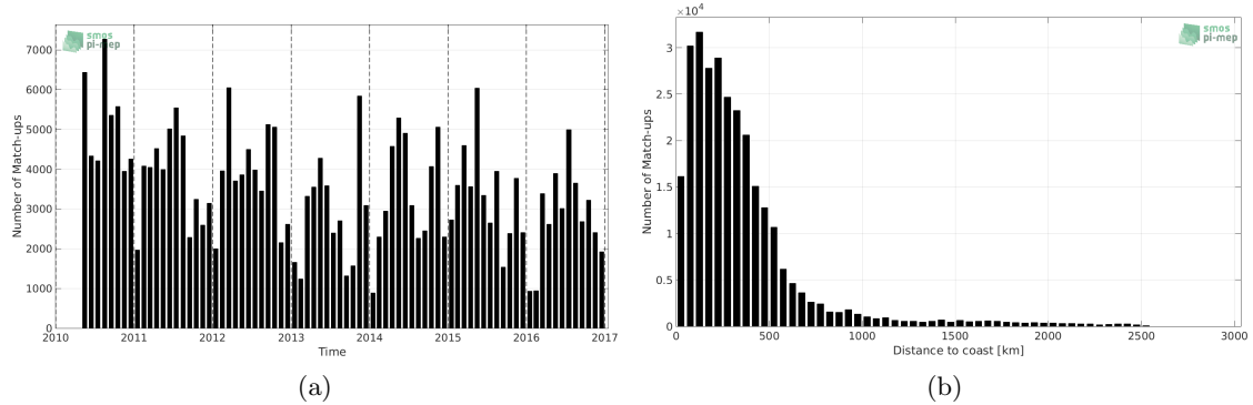
Figure 1: Number of match-ups between TSG-LEGOS-DM and SMOS-L3-CATDS-CECOS-IFREMER-V2-1DAY-0.5DEG SSS as a function of time (a) and as function of the distance to coast (b) over the Tropical Pacific Ocean Pi-MEP region and for the full satellite product period.
