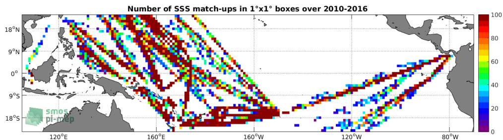
Figure 4: Number of SSS match-ups between TSG-LEGOS-DM SSS and the SMOS-L3-CATDS-CECOS-IFREMER-V2-1DAY-0.5DEG SSS product for the Tropical Pacific Ocean Pi-MEP region over 1^\circ \times 1^\circ boxes and for the full satellite product period.
