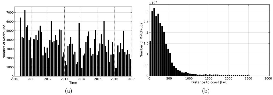
Figure 1: Number of match-ups between TSG-LEGOS-DM and SMOS-L3-CATDS-CECOS-IFREMER-V2-1DAY-0.5DEG SSS as a function of time (a) and as function of the distance to coast (b) over the Tropical Pacific Ocean Pi-MEP region and for the full satellite product period.
