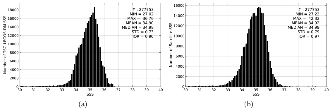
Figure 2: Histograms of SSS from TSG-LEGOS-DM (a) and SMOS-L3-CATDS-CECOS-IFREMER-V2-1DAY-0.5DEG (b) considering all match-up pairs per bins of 0.1 over the Tropical Pacific Ocean Pi-MEP region and for the full satellite product period.
