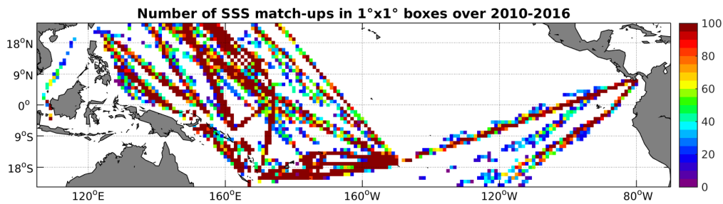
Figure 4: Number of SSS match-ups between TSG-LEGOS-DM SSS and the SMOS-L3-CATDS-CECOS-IFREMER-V2-1DAY-0.5DEG SSS product for the Tropical Pacific Ocean Pi-MEP region over 1^\circ \times 1^\circ boxes and for the full satellite product period.
