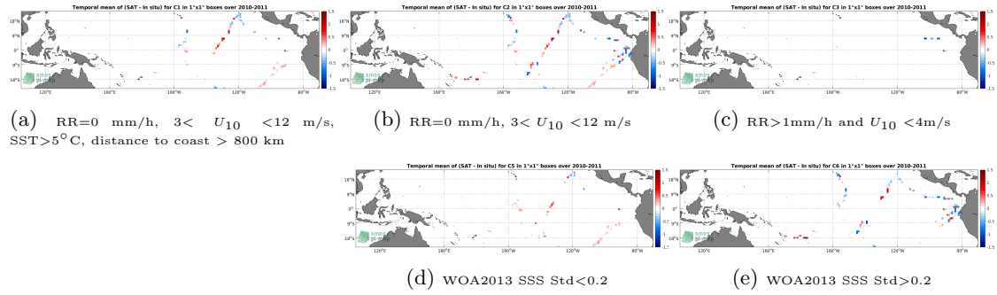
Figure 12: Temporal mean gridded over spatial boxes of size 1^{\circ}\times 1^{\circ} of \Delta SSS (SMOS SSS L3 v2 - Daily - 0.5 Deg (CATDS-CECOS-IFREMER) - TSG (GOSUD-Sailing-ship)) for 5 different subdatasets corresponding to:RR=0 mm/h, 3 < U_{10} < 12 m/s, SST >5^{\circ}\text{C} , distance to coast > 800 km (a), RR=0 mm/h, 3 < U_{10} < 12 m/s (b), RR >1 mm/h and U_{10} < 4 m/s (c), WOA2013 SSS Std <0.2 (d), WOA2013 SSS Std >0.2 (e).
