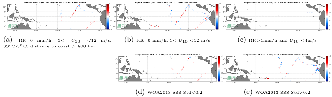
Figure 12: Temporal mean gridded over spatial boxes of size 1^{\circ}\times 1^{\circ} of \Delta SSS (SMOS L3 v2 - Daily - 0.5 Deg (CATDS-CECOS-IFREMER) - TSG-GOSUD-Sailing-ship) for 5 different subdatasets corresponding to:RR=0 mm/h, 3 < U_{10} < 12 m/s, SST >5^{\circ}\text{C} , distance to coast > 800 km (a), RR=0 mm/h, 3 < U_{10} < 12 m/s (b), RR >1 mm/h and U_{10} < 4 m/s (c), WOA2013 SSS Std <0.2 (d), WOA2013 SSS Std >0.2 (e).
