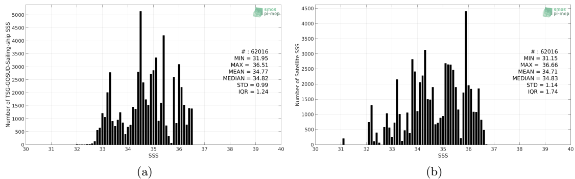
Figure 2: Histograms of SSS from TSG-GOSUD-Sailing-ship (a) and SMOS L3 v2 - Daily - 0.5 Deg (CATDS-CECOS-IFREMER) (b) considering all match-up pairs per bins of 0.1 over the Tropical Pacific Ocean Pi-MEP region and for the full satellite product period.
