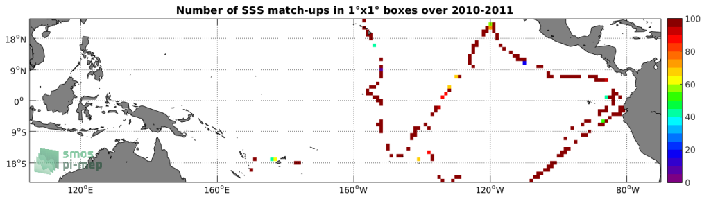
Figure 4: Number of SSS match-ups between TSG-GOSUD-Sailing-ship SSS and the SMOS L3 v2 - Daily - 0.5 Deg (CATDS-CECOS-IFREMER) SSS product for the Tropical Pacific Ocean Pi-MEP region over 1^\circ \times 1^\circ boxes and for the full satellite product period.
