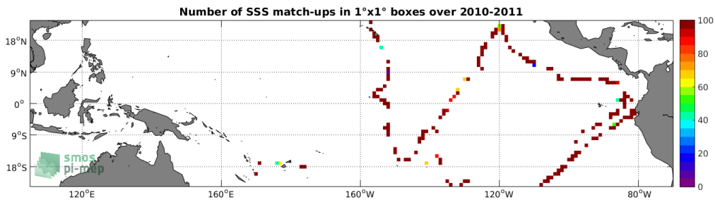
Figure 4: Number of SSS match-ups between TSG-GOSUD-Sailing-ship SSS and the SMOS-L3-CATDS-CECOS-IFREMER-V2-1DAY-0.5DEG SSS product for the Tropical Pacific Ocean Pi-MEP region over 1^\circ \times 1^\circ boxes and for the full satellite product period.
