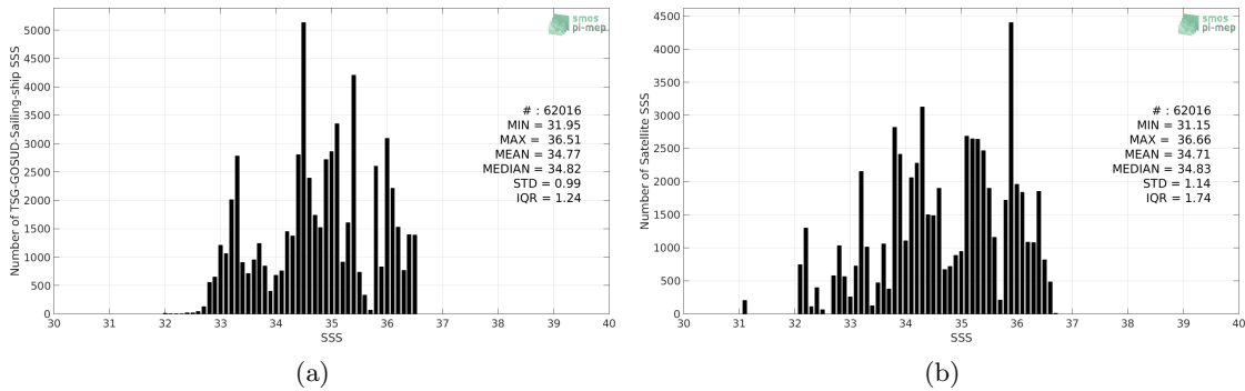
Figure 2: Histograms of SSS from TSG-GOSUD-Sailing-ship (a) and SMOS-L3-CATDS-CECOS-IFREMER-V2-1DAY-0.5DEG (b) considering all match-up pairs per bins of 0.1 over the Tropical Pacific Ocean Pi-MEP region and for the full satellite product period.
